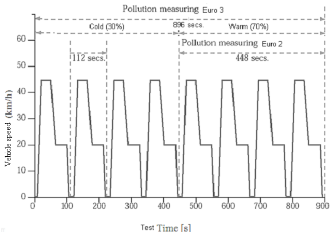
Figure 1: Pollutant emission sampling for Euro 3 as compared to with Euro 2 for an L1e, L2e or L6e category vehicle.
