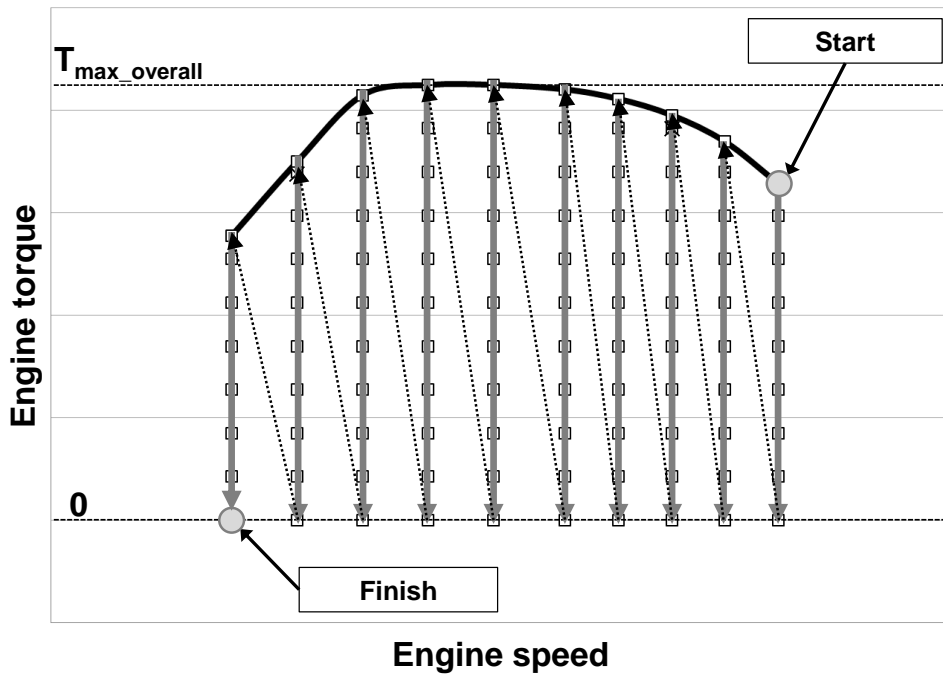
Figure 4: Sequence of steady state measurement setpoints
