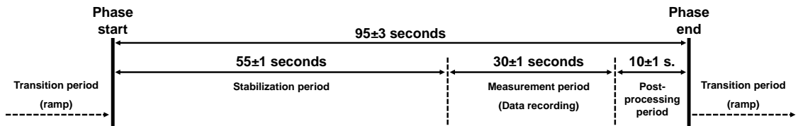
Figure 3: Steps to be performed at each measurement setpoint
