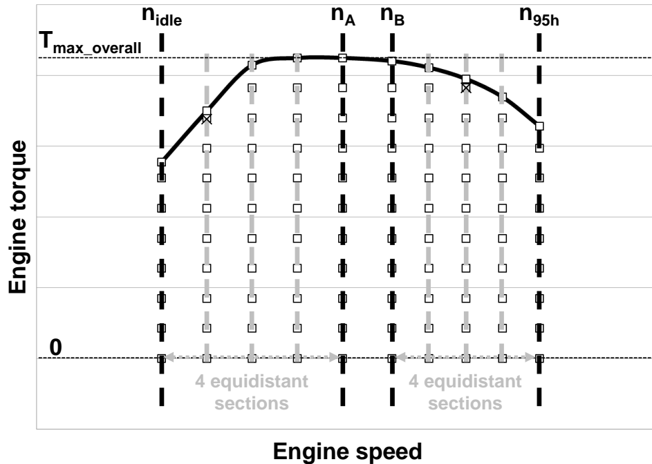
Figure 1: Definition of speed setpoints
