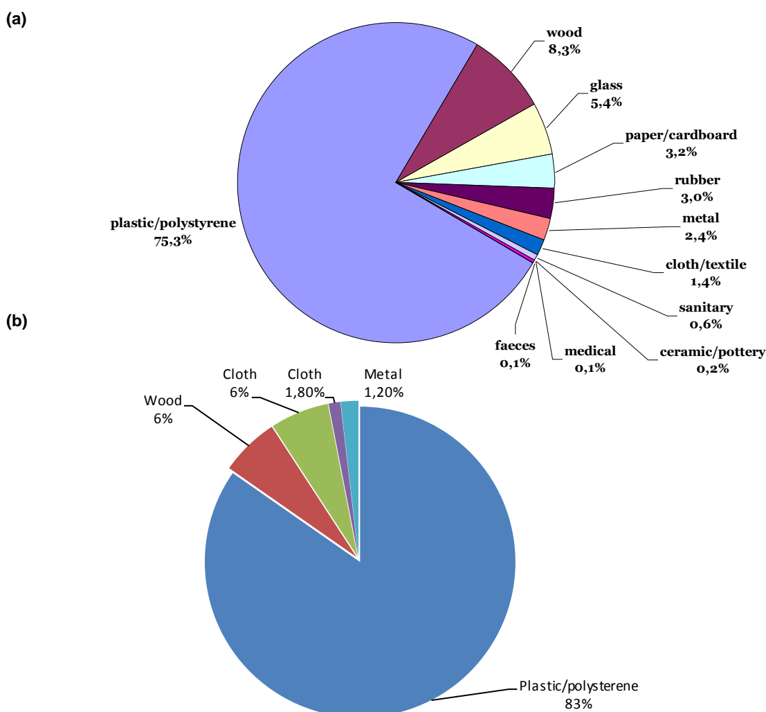
Fig. 13. Composition based on the number of items of marine litter collected during (a) the OSPAR “Beach Litter Monitoring Program” along the southern North Sea coast (2002-2008); (b) the ICC campaign in the Mediterranean (2002-2006).
