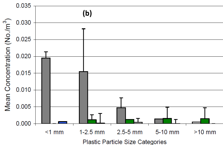
Fig. 7. Abundance of plastic particles (mean \pm SE) according to plastic particle size categories in samples, combined from (a) Bering Sea cruises (2006), and (b) US west coast cruises (2006-2007).
