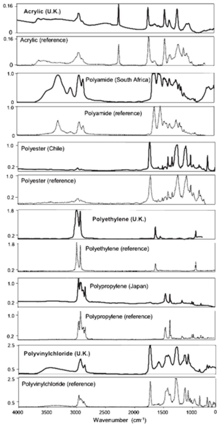
Fig. 12. Examples of Fourier transform infrared spectra of microplastic and corresponding reference material from ATR spectral database, vertical axis represents transmission in standard optical density units. (Bruker Optics ATR-Polymer Library - a Collection of Synthetic Fibres, Copyright 2004 Bruker Optic GmbH). From Browne et al., 2011.
