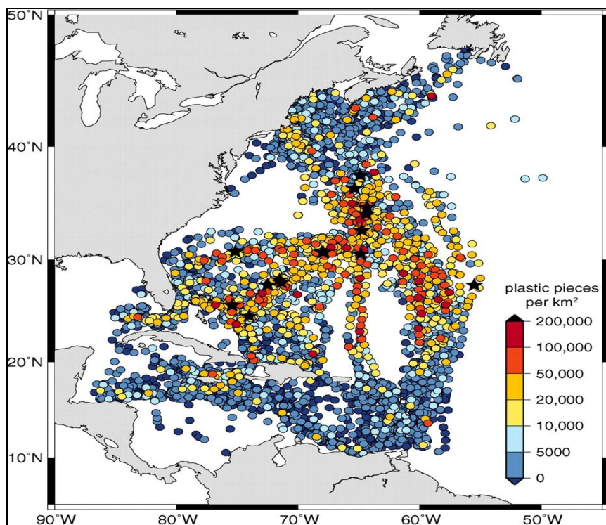
Fig. 9. Distribution of plastic marine litter collected in 6136 surface plankton net tows (1.0 x 0.5 m mouth with a 335 \mu\text{m} mesh net) on annually repeated cruise tracks from 1986 to 2008 in the western North Atlantic Ocean and Caribbean Sea. Black stars indicate tows with measured concentration greater than 200,000 pieces per \text{km}^2 (Law et al. 2010).
