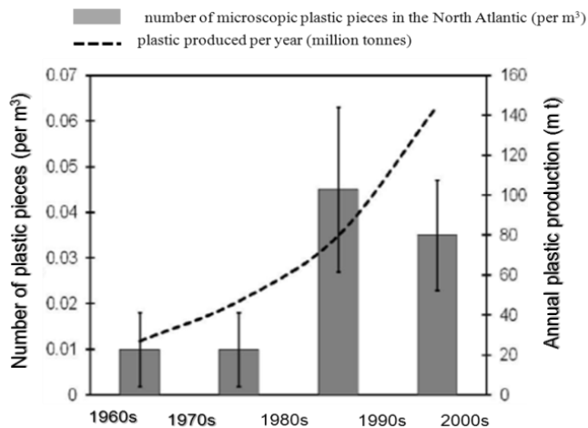
Fig. 11. Microscopic plastics (< 5 mm) in surface waters, collected with continuous plankton recorder and identified by FT-IR, revealed a significant increase in abundance when samples from the 1960s and 1970s were compared with the 1980s and 1990s ( F_{3,3} = 14.42 , p < 0.05 ) (modified after Thompson et al., 2004).
