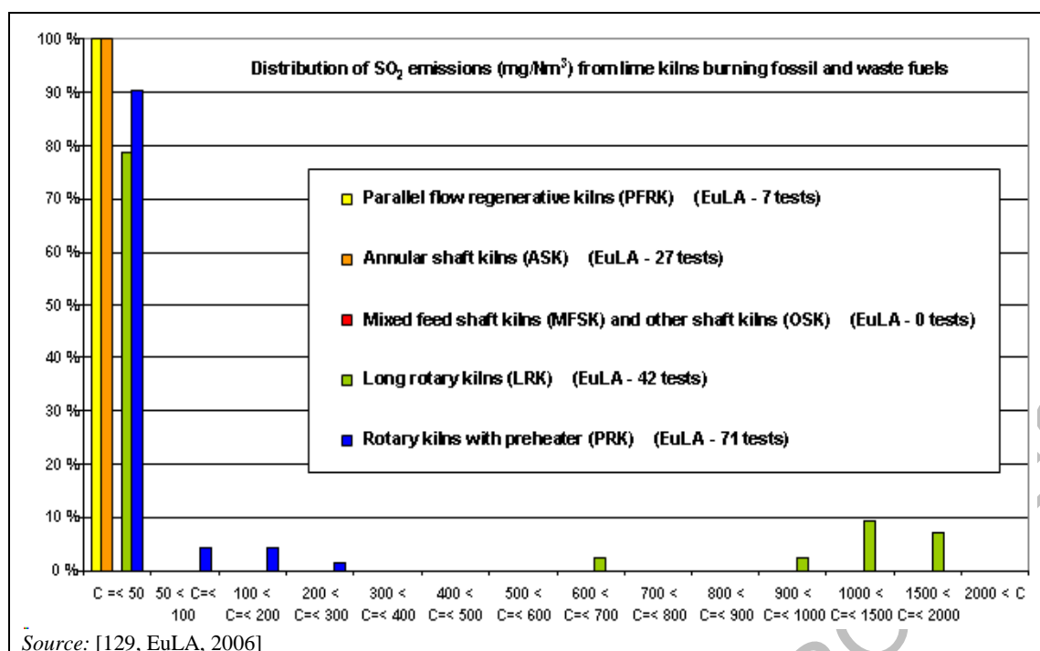
Figure 2.38: SO 2 emissions measured from different types of lime kilns using fossil fuels and waste fuels for kin firing in the EU-27 (spot measurements as half hourly values)
