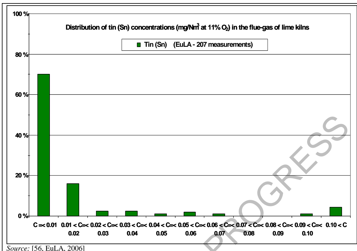
Figure 6.21: Distribution of tin concentrations in the flue-gas of lime kilns in the EU-27
