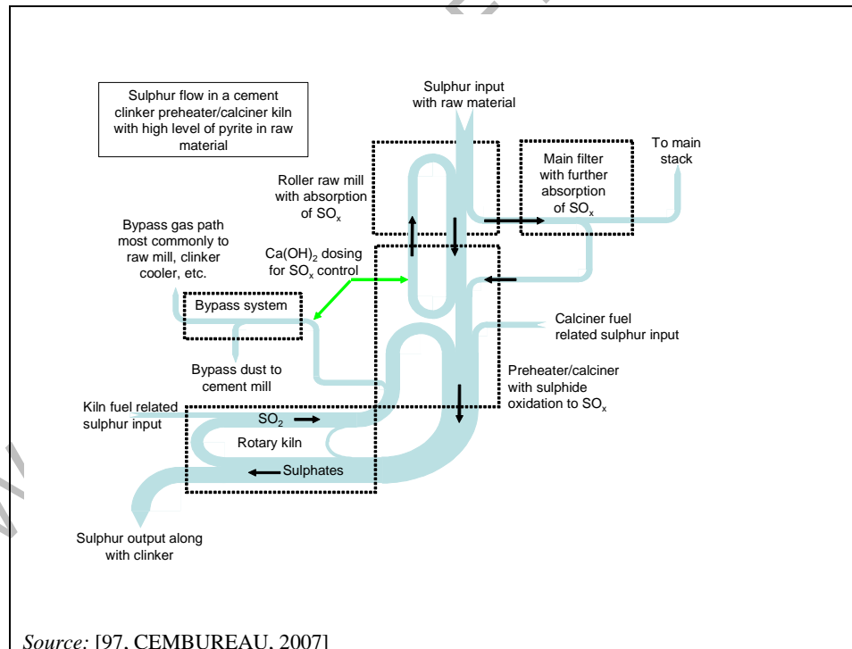
Figure 1.31: Sulphur flow diagram in a cement preheater/precalciner kiln
