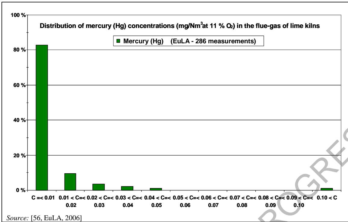
Figure 6.15: Distribution of mercury concentrations in the flue-gas of lime kilns in the EU-27
