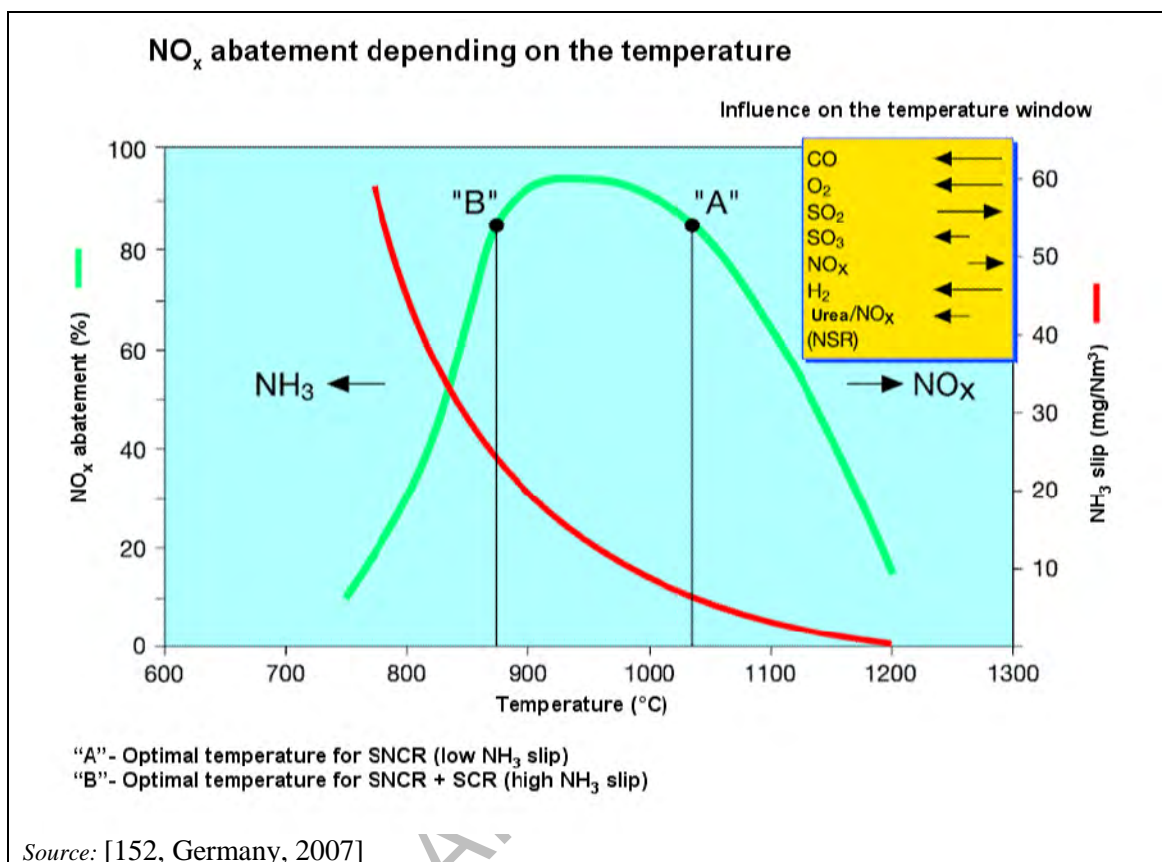
Figure 2.50: NO x abatement depending on the temperature
