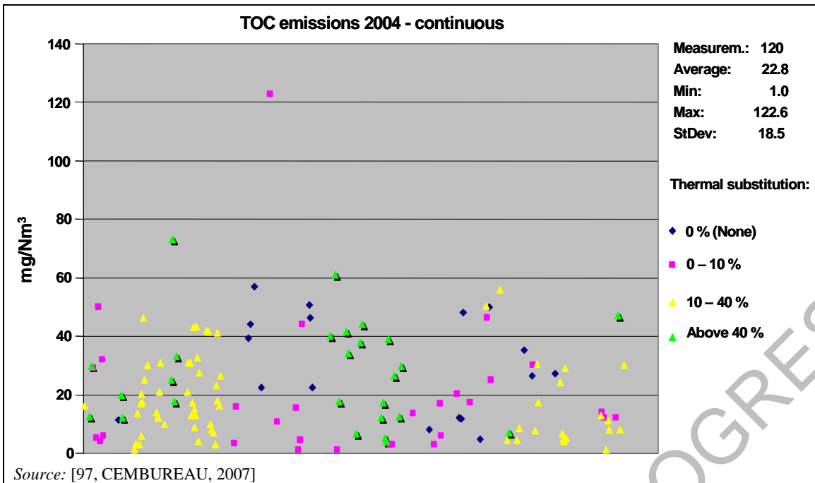
Figure 1.35: TOC emission values from continuous measurements in the clean gas of cement kilns in the EU-27 and EU-23+ countries
