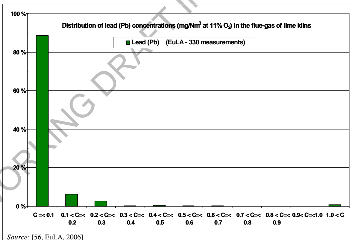
Figure 6.18: Distribution of lead concentrations in the flue-gas of lime kilns in the EU-27
