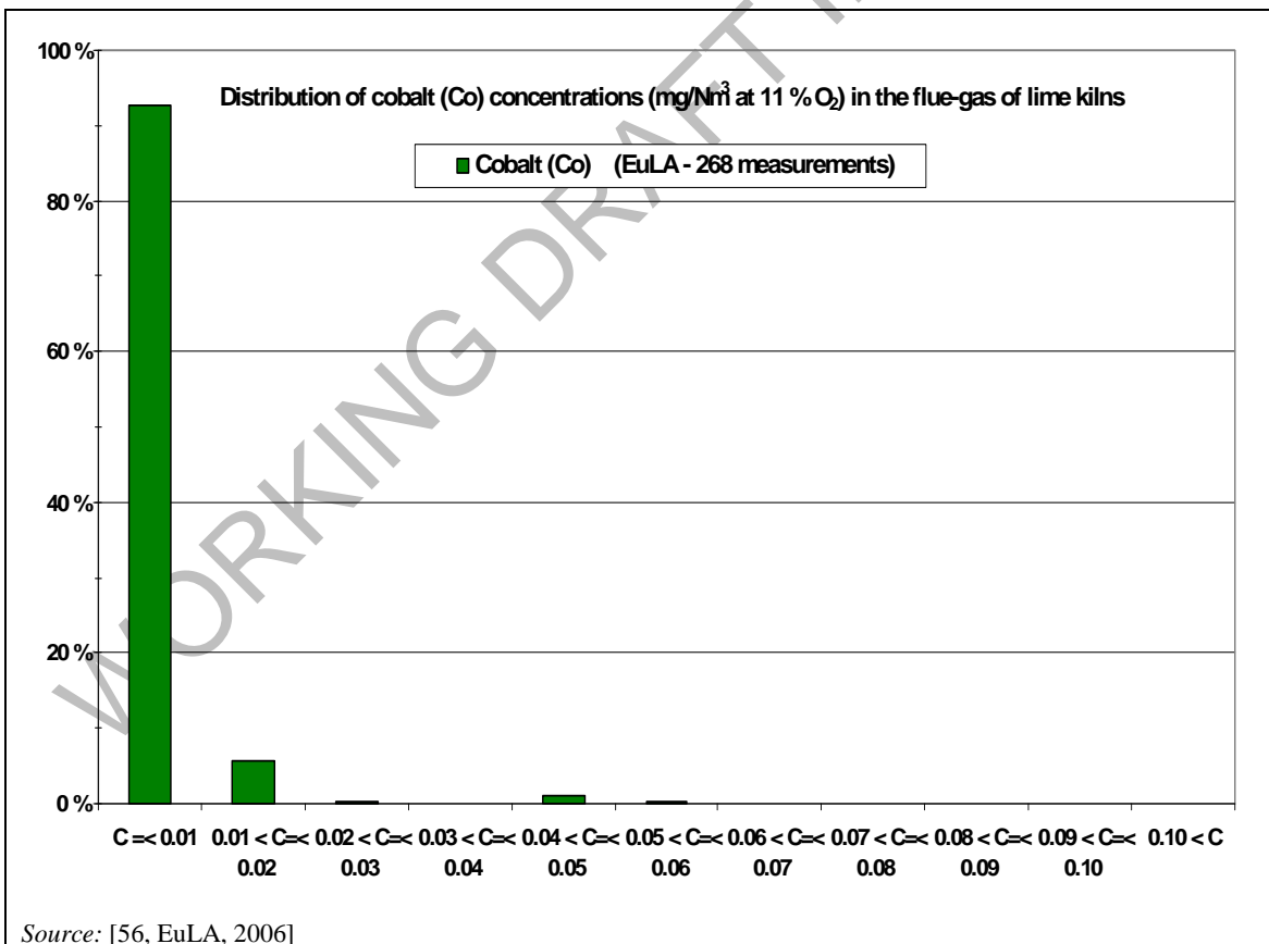
Figure 6.12: Distribution of cobalt concentrations in the flue-gas of lime kilns in the EU-27
