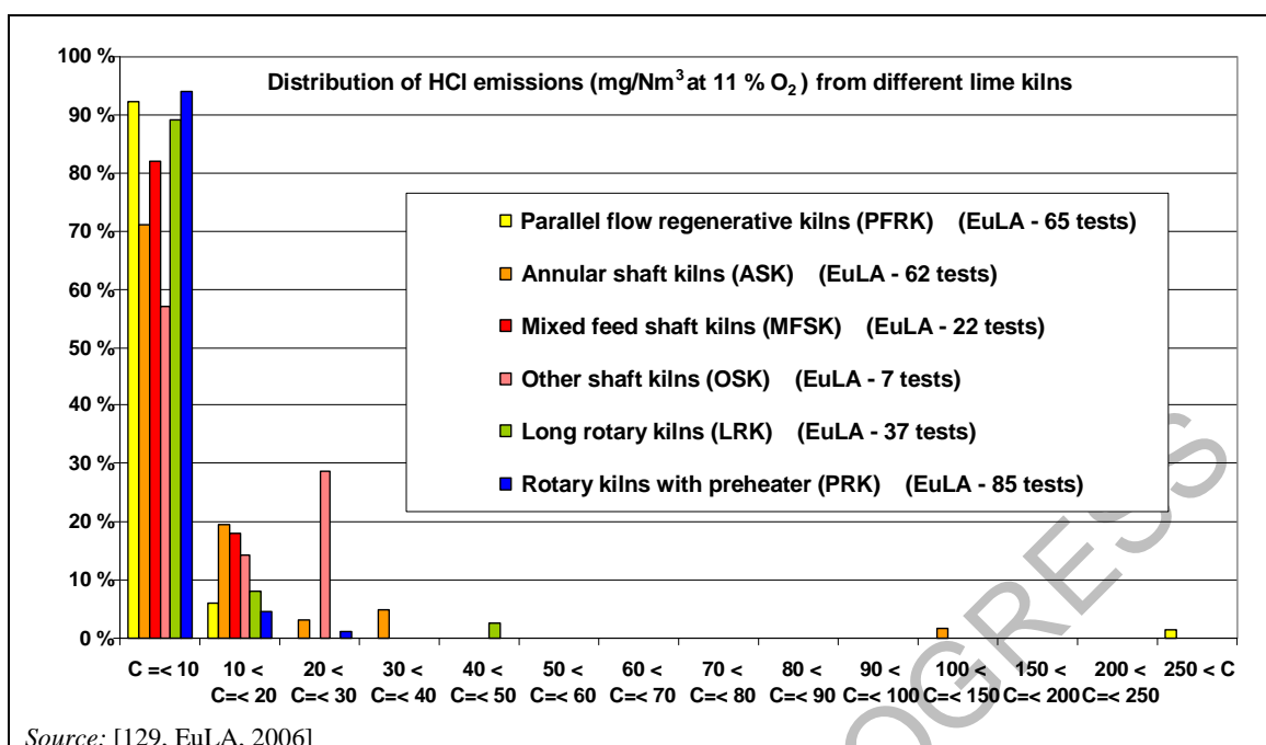
Figure 2.42: HCl emissions from different lime kilns in the EU-27
