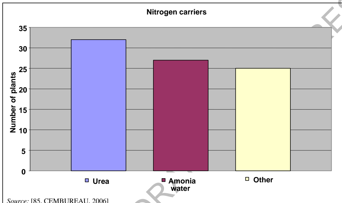
Figure 1.65: Nitrogen carriers/NH 2 -X agents used by SNCR in EU-23+ countries
