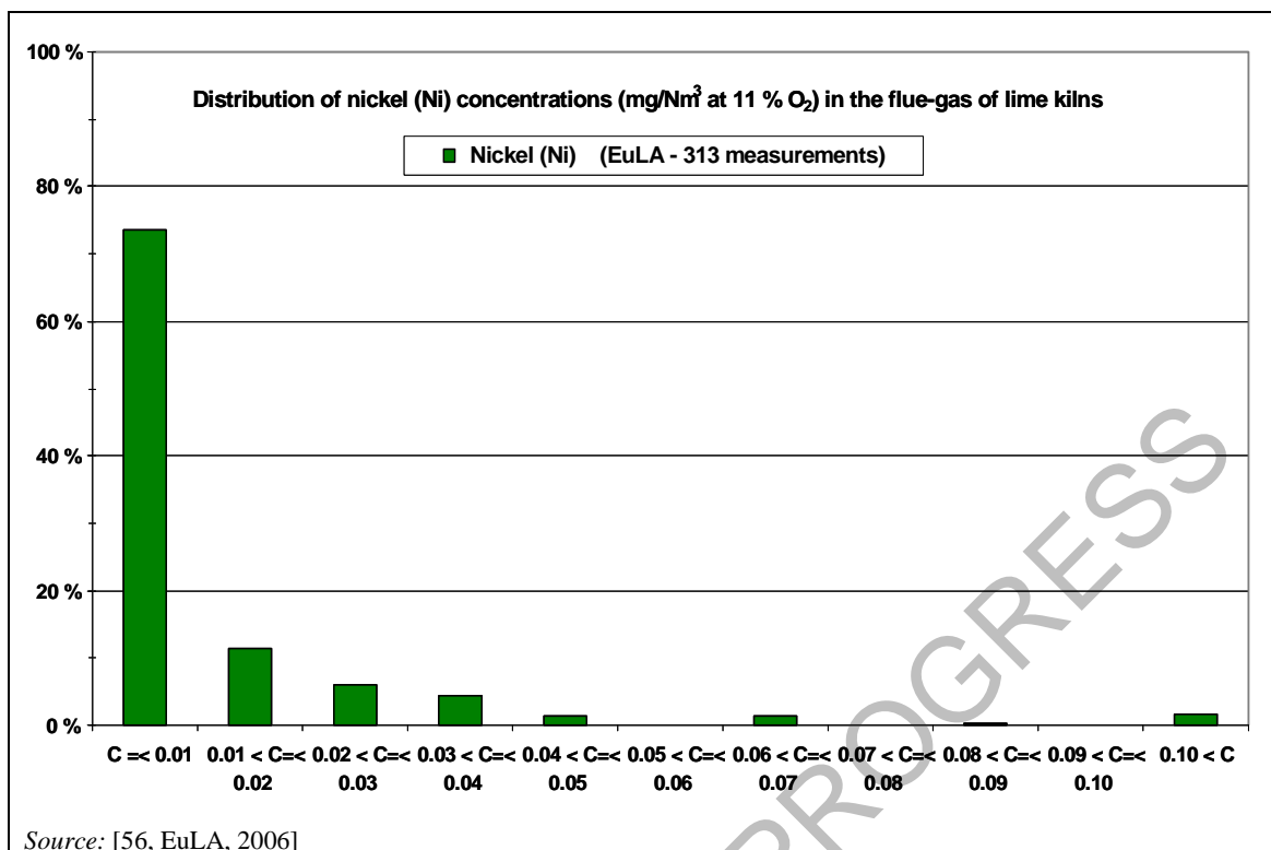
Figure 6.17: Distribution of nickel concentrations in the flue-gas of lime kilns in the EU-27
