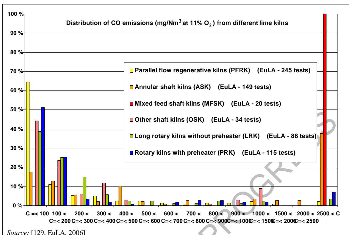
Figure 2.39: CO emissions occurring from different types of lime kilns in the EU-27
