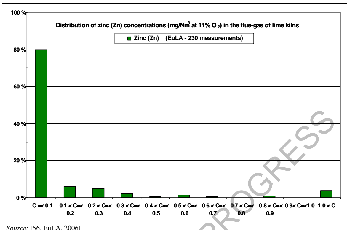
Figure 6.25: Distribution of zinc concentrations in the flue-gas of lime kilns in the EU-27
