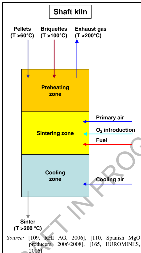
Figure 3.11: Operating principle of shaft kilns in magnesia production
