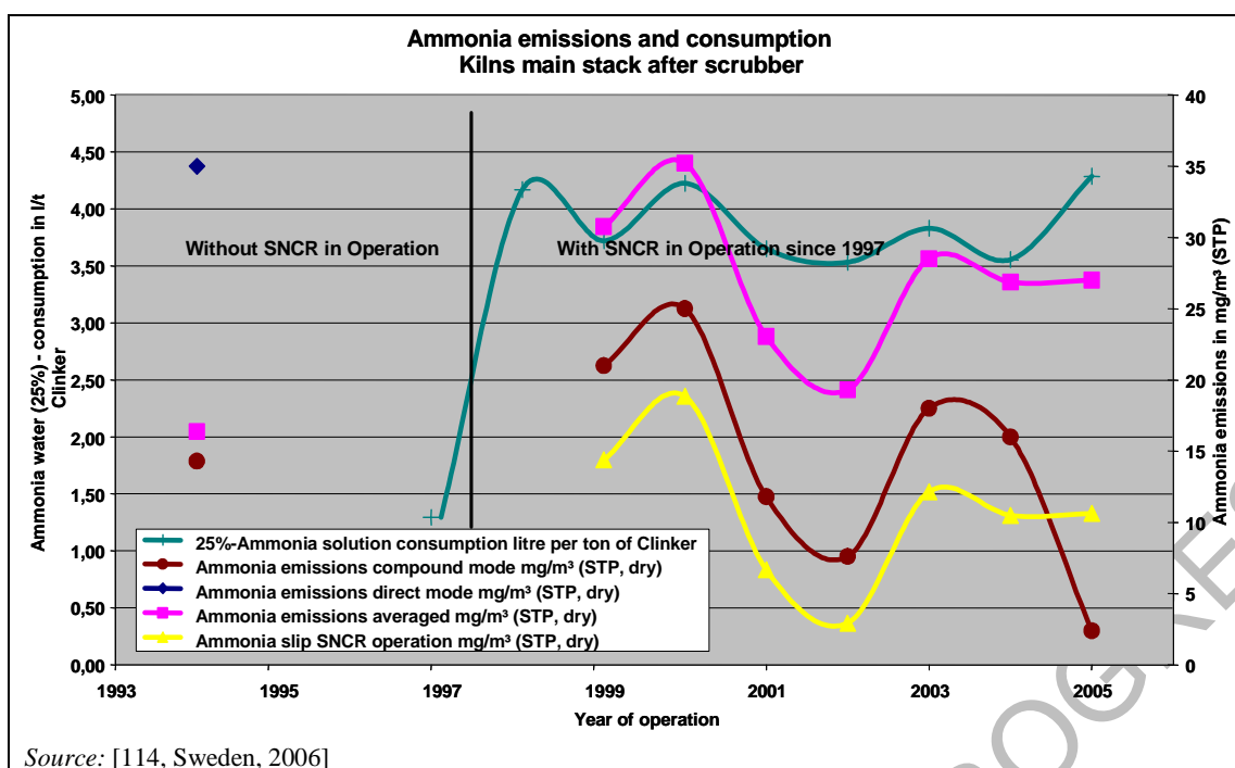
Figure 1.58: Ammonia emissions from a Swedish cement plant equipped with a \text{SO}_x scrubber
