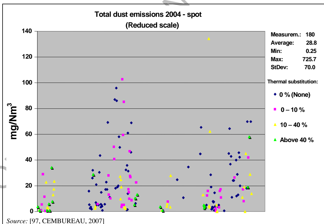
Figure 1.24: Dust emission values from 180 spot dust measurements in the clean gas of rotary kilns in the EU-27 and EU 23+ countries
