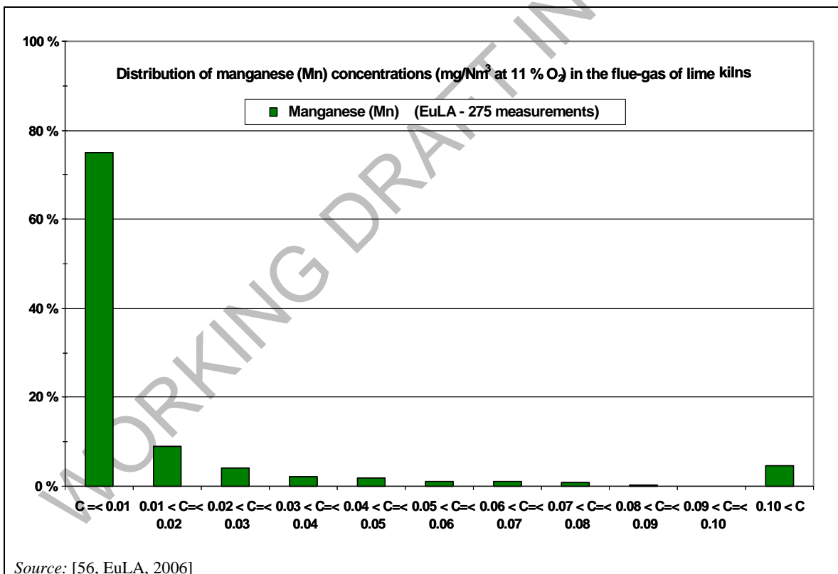
Figure 6.16: Distribution of manganese concentrations in the flue-gas of lime kilns in the EU-27
