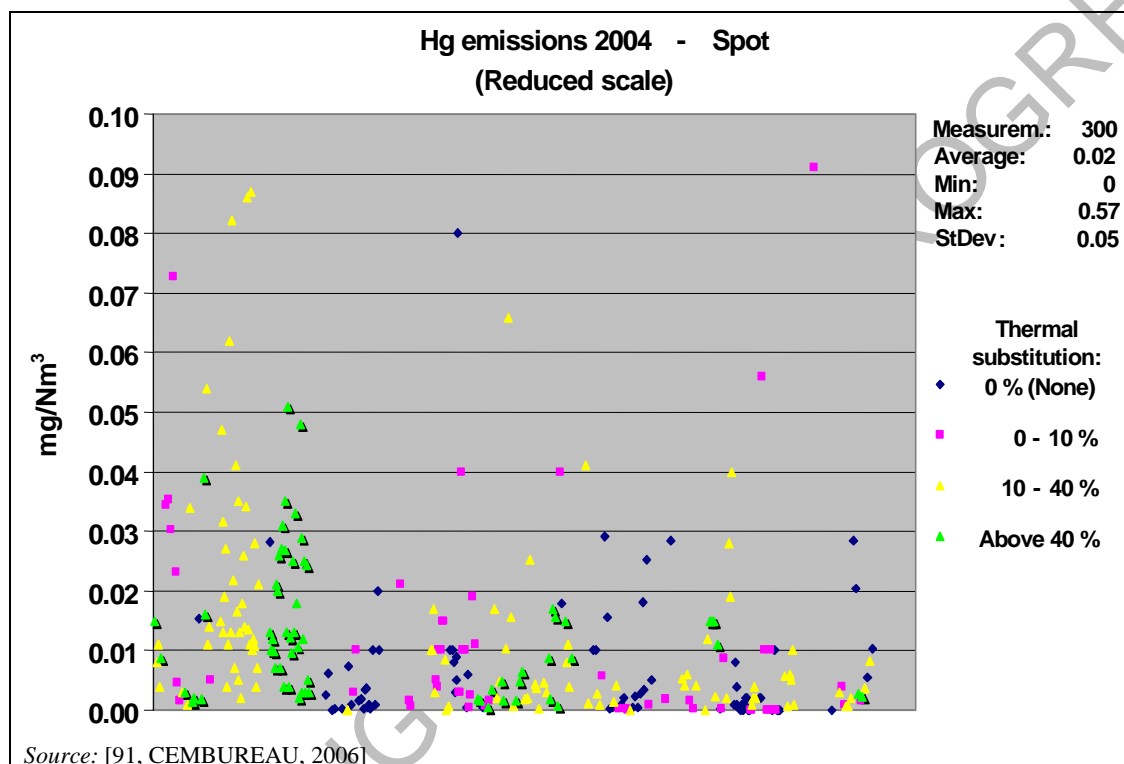
Figure 1.46: Mercury emission values from 306 spot Hg measurements in the EU-27 and EU-23+ countries
