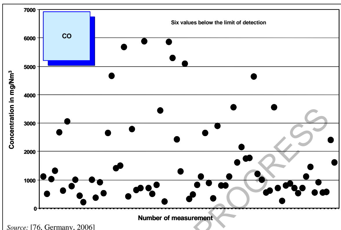
Figure 1.34: CO emissions concentration values measured in the clean gas from 29 German rotary kilns in 2004
