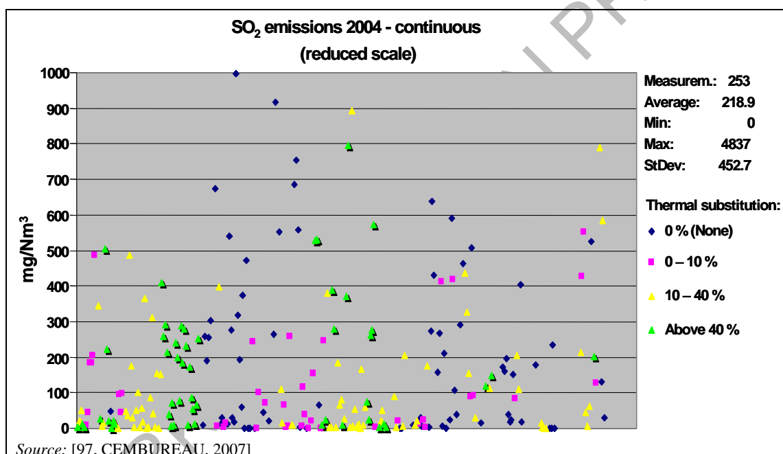
Figure 1.32: Values of SO 2 measurements in the clean gas from cement plants in the EU-27 and EU-23+ countries
