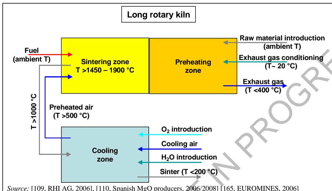
Figure 3.10: Operating principle of long rotary kilns in magnesia production
