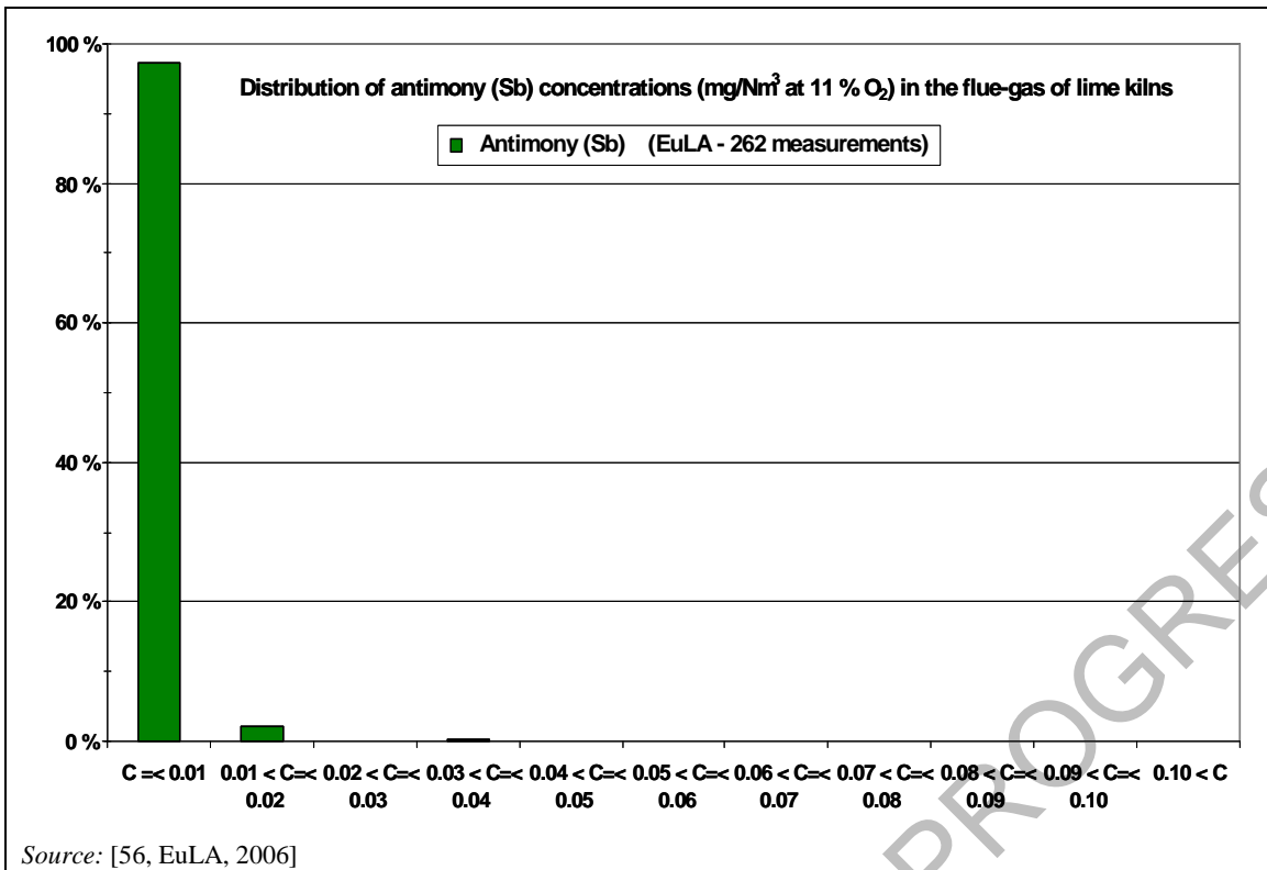
Figure 6.19: Distribution of antimony concentrations in the flue-gas of lime kilns in the EU-27
