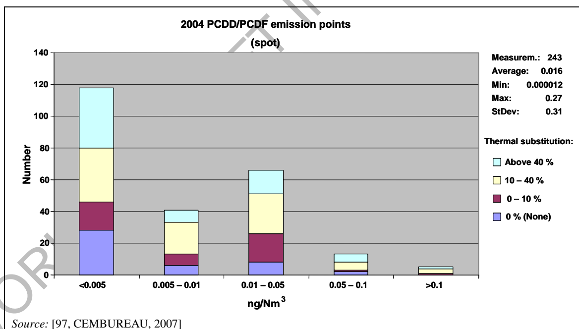
Figure 1.39: Distribution of spot measurements categorised by the thermal substitution rate of PCDD/F levels from cement kilns in the EU-27 and EU-23+ countries
