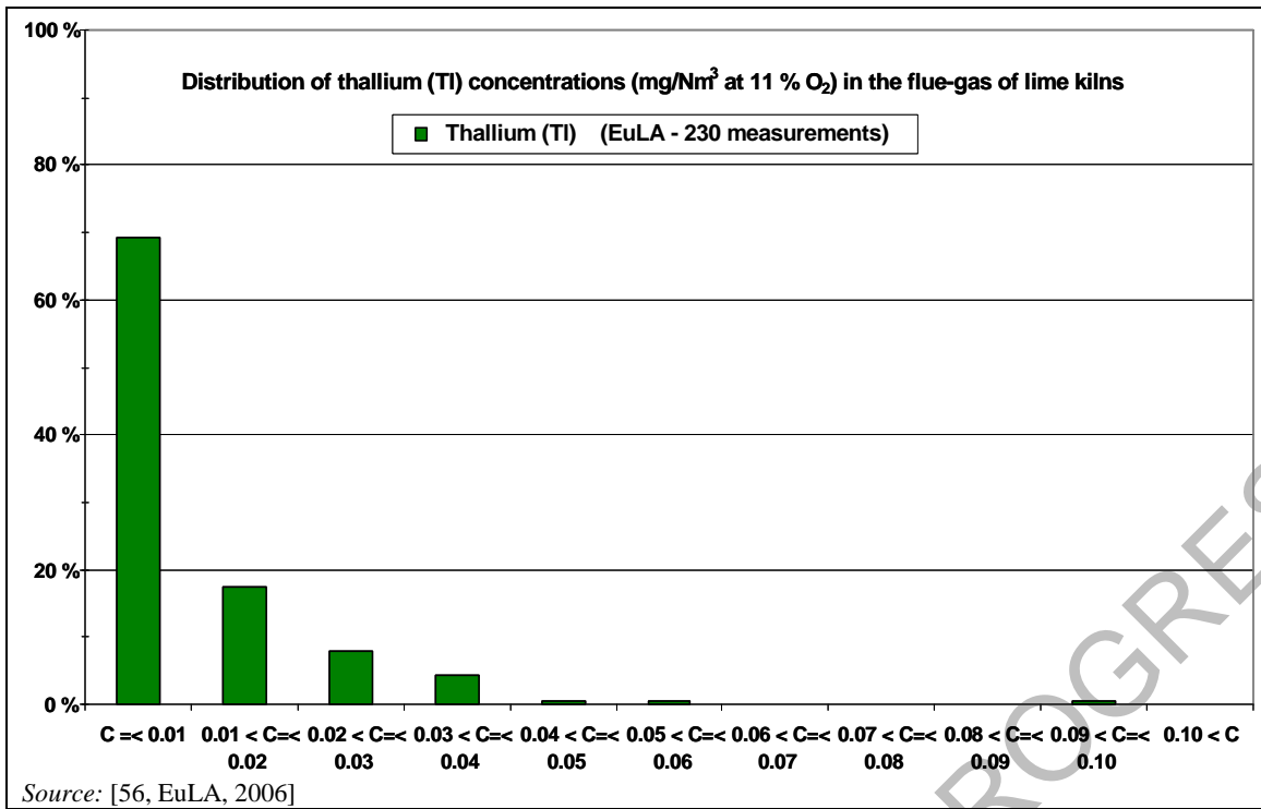
Figure 6.23: Distribution of thallium concentrations in the flue-gas of lime kilns in the EU-27
