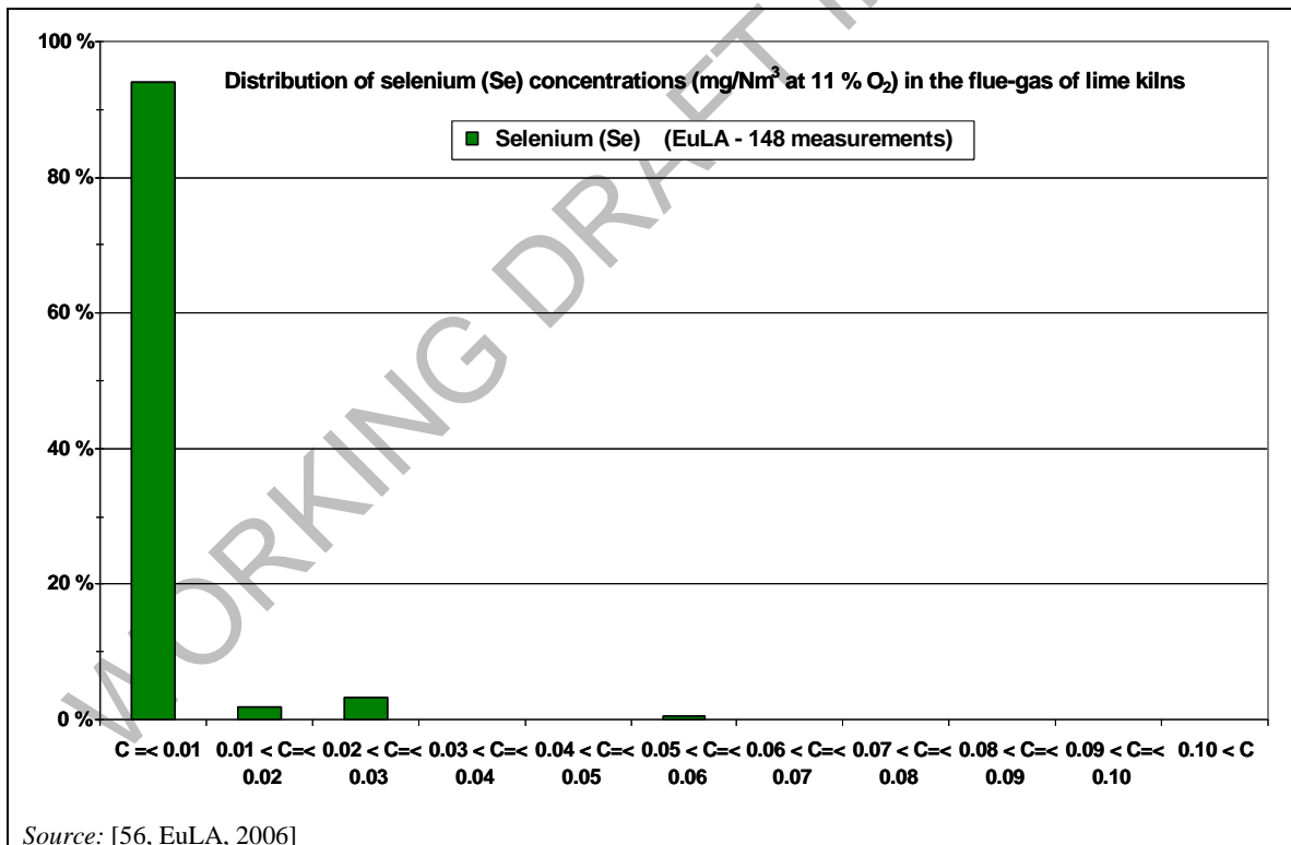
Figure 6.20: Distribution of selenium concentrations in the flue-gas of lime kilns in the EU-27
