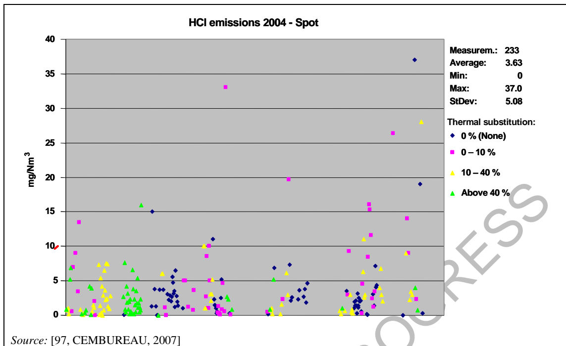
Figure 1.50: Emission values from 233 spot measurements in the clean gas of rotary kilns in the EU-27 and EU-23+ countries
