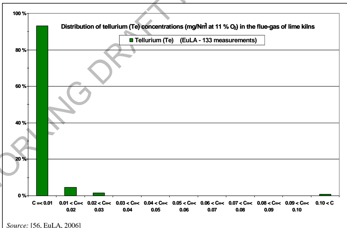
Figure 6.22: Distribution of tellurium concentrations in the flue-gas of lime kilns in the EU-27
