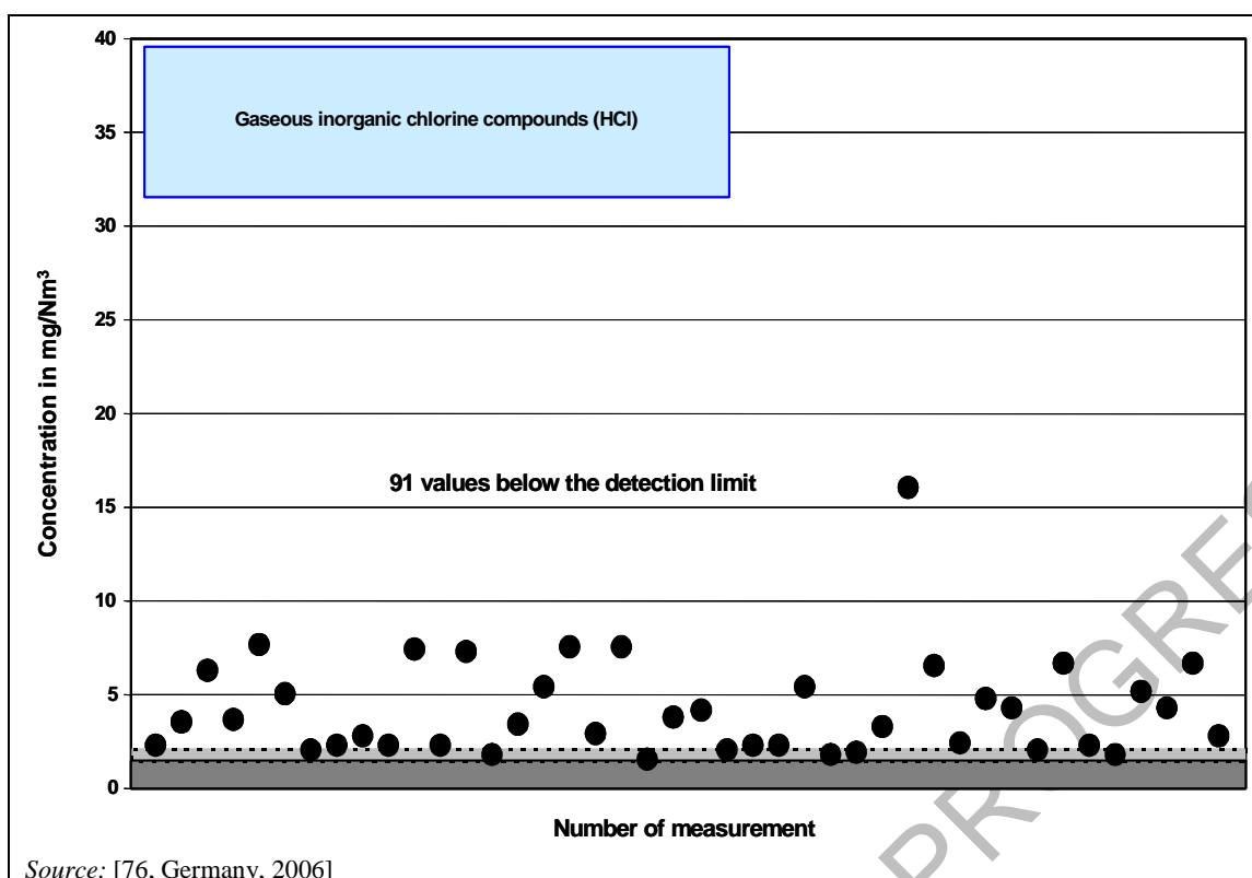
Figure 1.52: Emissions of gaseous inorganic chlorine compounds, stated as HCl, measured in the clean gas from 38 German rotary kilns in 2004
