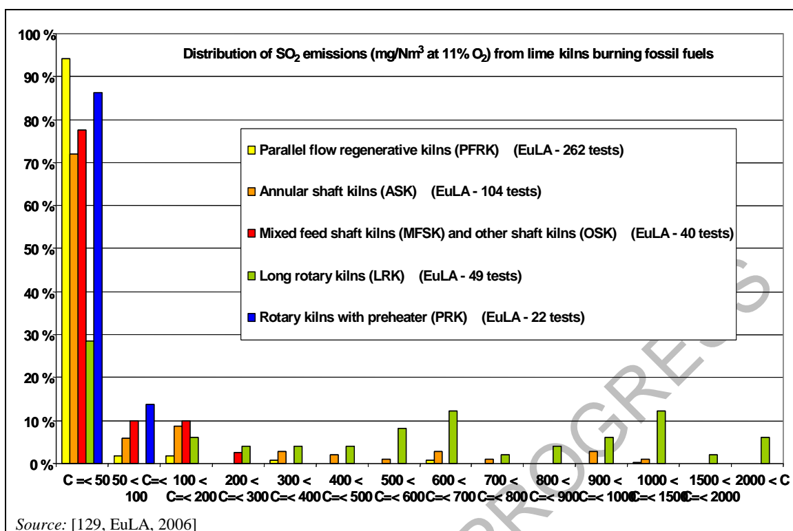
Figure 2.37: SO 2 emissions measured from different types of lime kilns using fossil fuels in the EU-27 (spot measurements as half hourly values)
