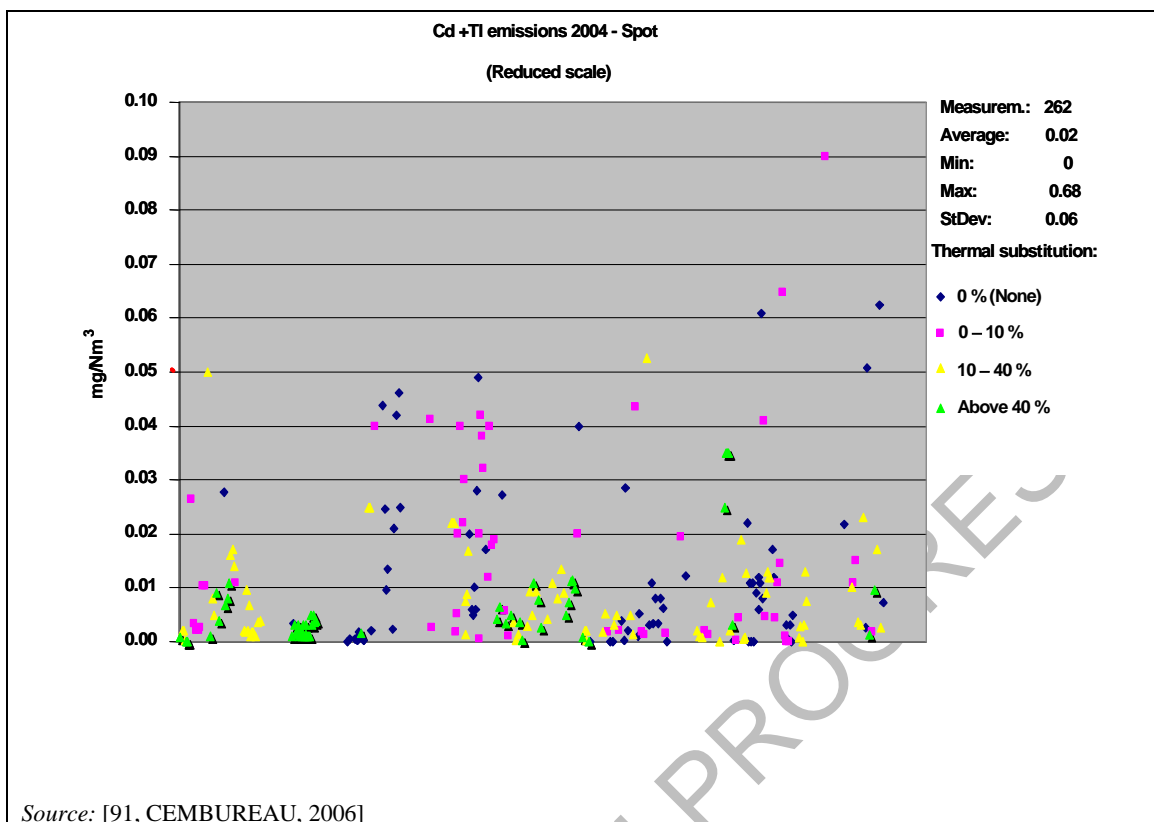
Figure 1.42: Cadmium and thallium emission values from 262 spot \Sigma (Cd, Tl) measurements in the EU-27 and EU-23+ countries
