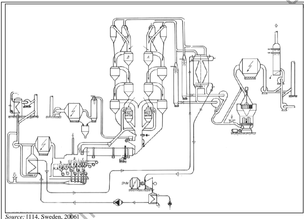
Figure 6.3: Flow diagram of the cement manufacturing process in Slite (Sweden)
