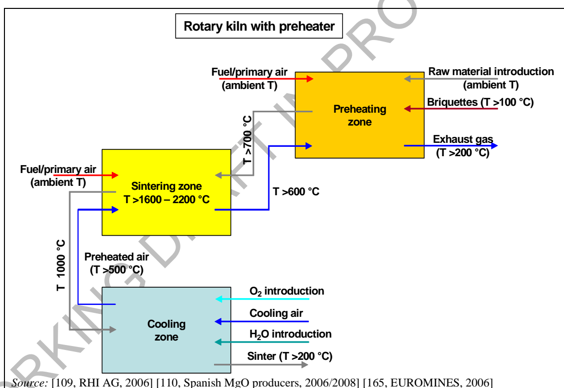
Figure 3.9: Operating principle of rotary kilns with a preheater in magnesia production
