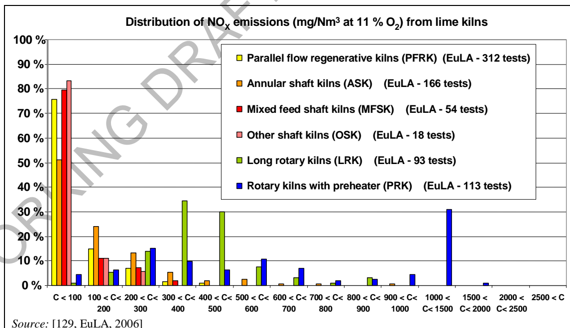
Figure 2.36: NO x emissions measured from different types of lime kilns in the EU-27 (spot measurements as half hourly values)
