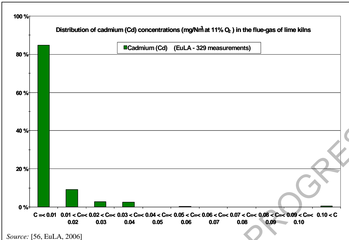
Figure 6.11: Distribution of cadmium concentrations in the flue-gas of lime kilns in the EU-27
