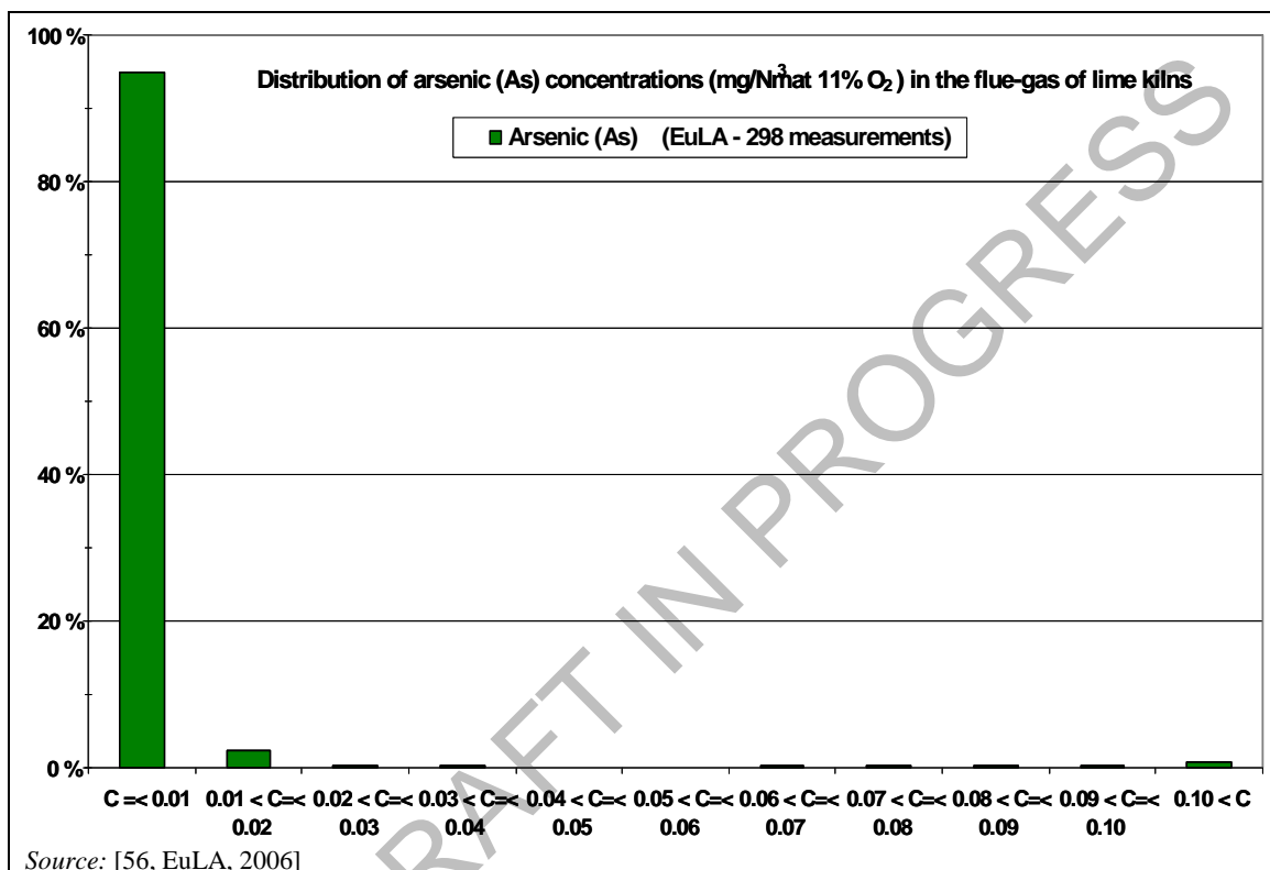
Figure 6.10: Distribution of arsenic concentrations in the flue-gas of lime kilns in the EU-27
