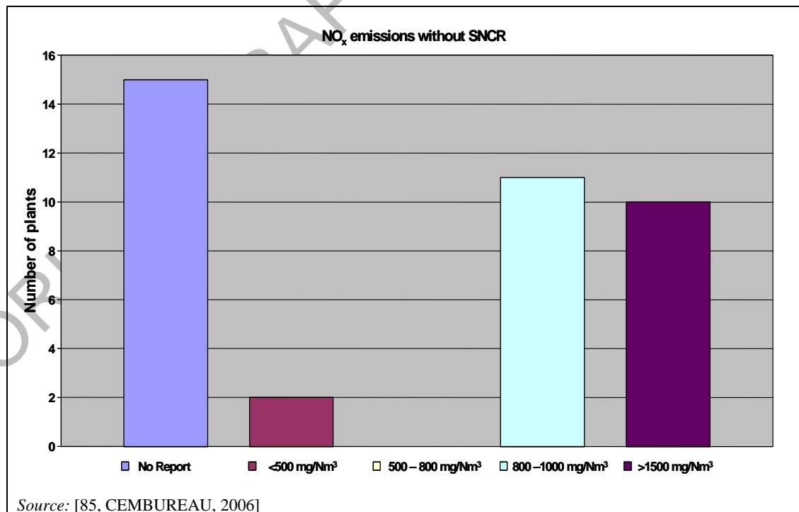
Figure 1.30: NO x emissions ranges achieved by several cement plants without using SNCR
