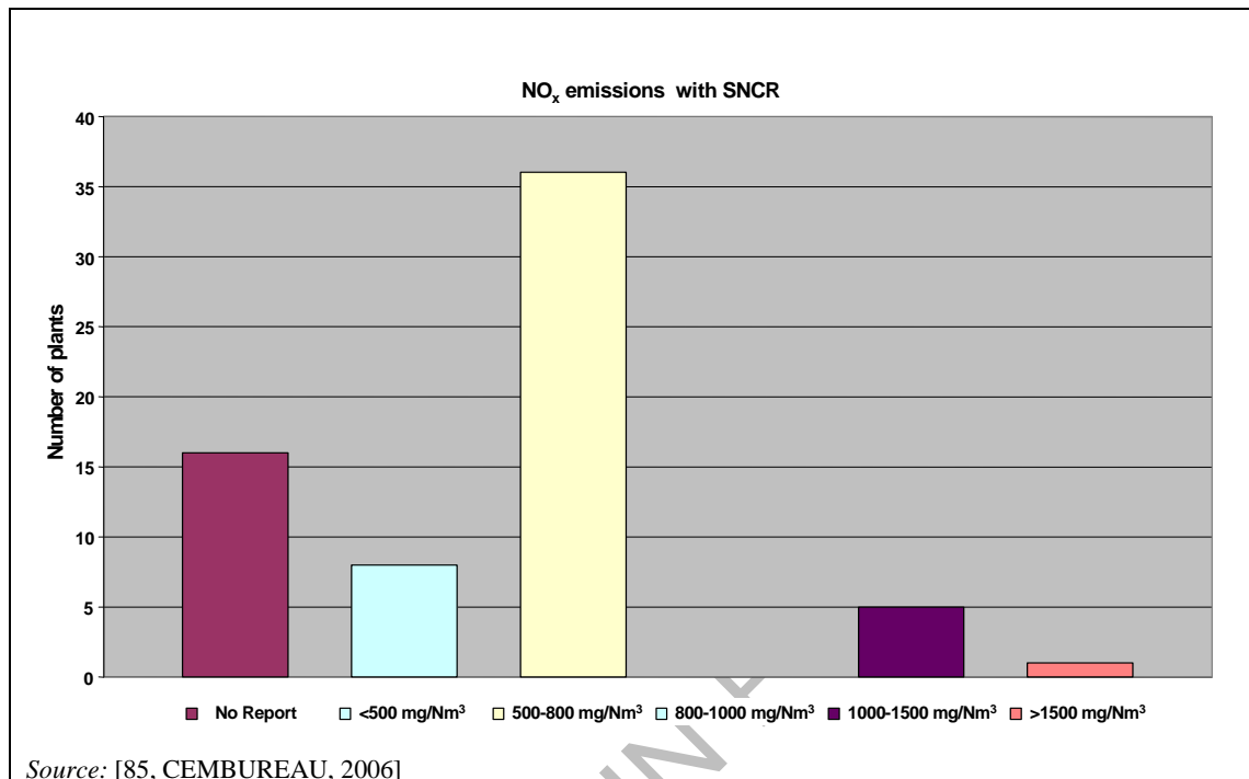
Figure 1.29: NO x emissions achieved by several cement plants using SNCR for NO x reduction
