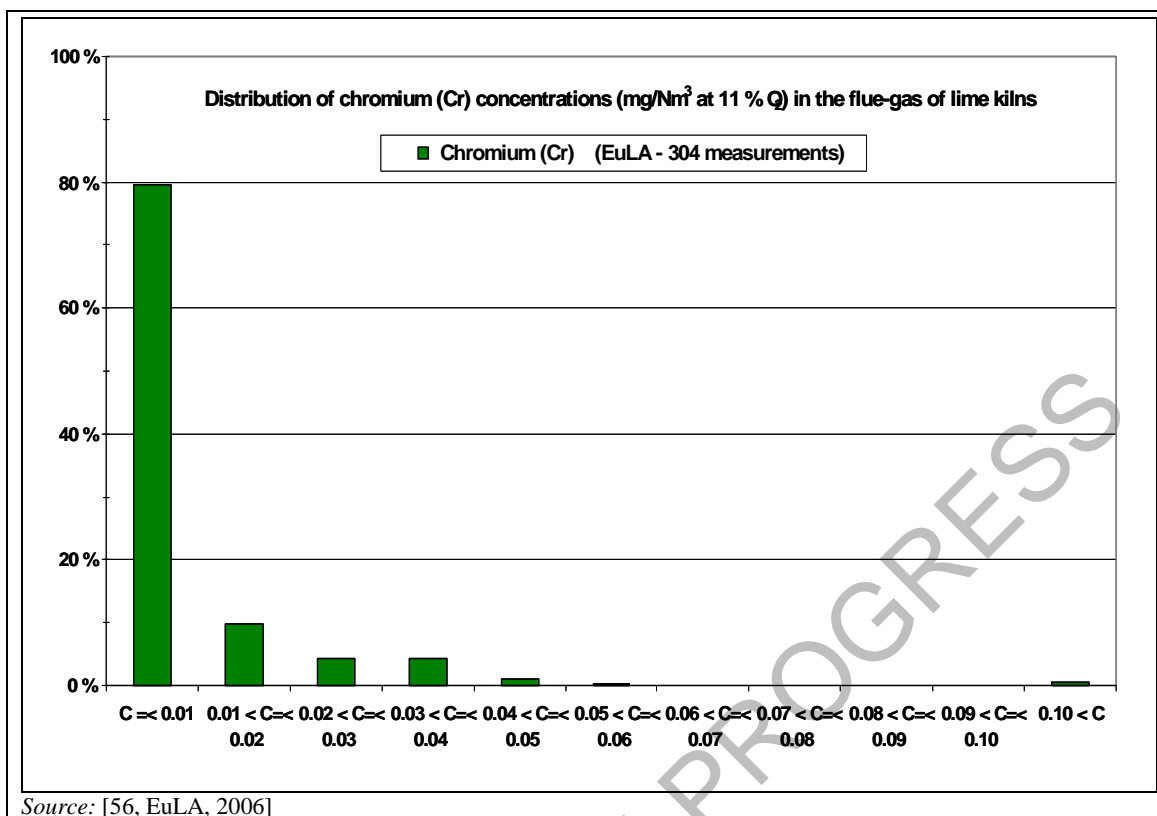
Figure 6.13: Distribution of chromium concentrations in the flue-gas of lime kilns in the EU-27
