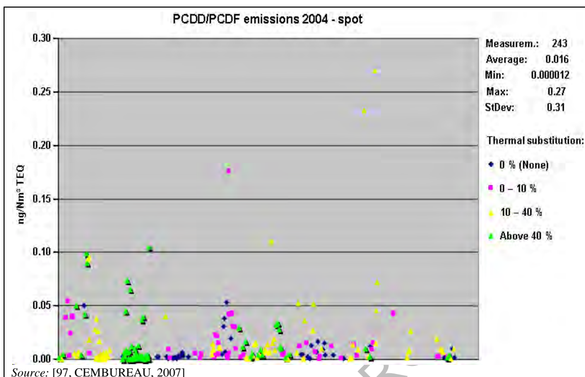
Figure 1.38: Emissions of PCDD/F in the EU-27 and EU-23+ countries in 2004 categorised by thermal substitution rate
