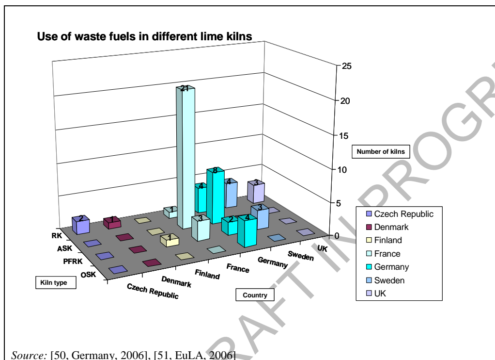
Figure 2.13: Distribution of lime kilns using waste fuels in different European countries
