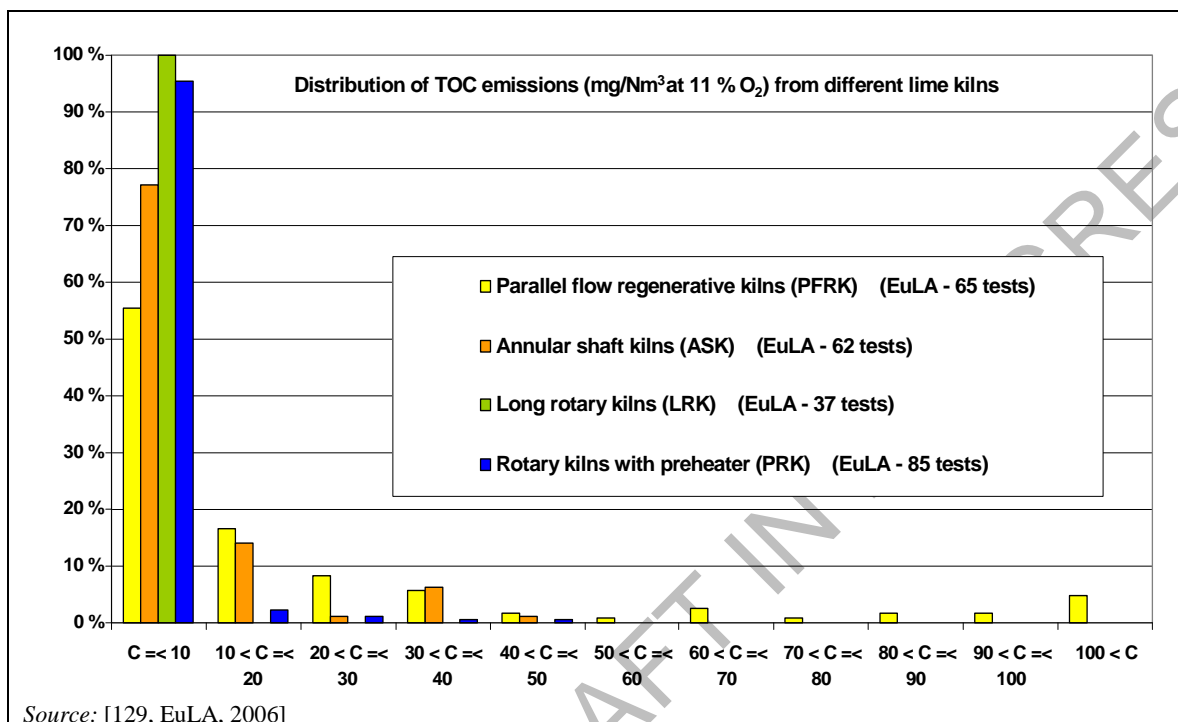
Figure 2.41: TOC emissions occurring from different types of lime kilns in the EU-27
