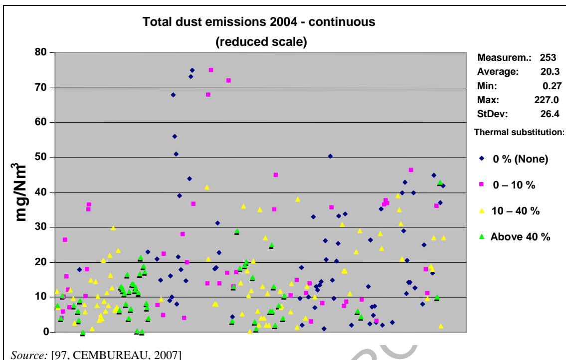
Figure 1.23: Ranges of emission values from continuous dust measurements in the clean gas from 253 rotary kilns in the EU-27 and EU 23+ countries
