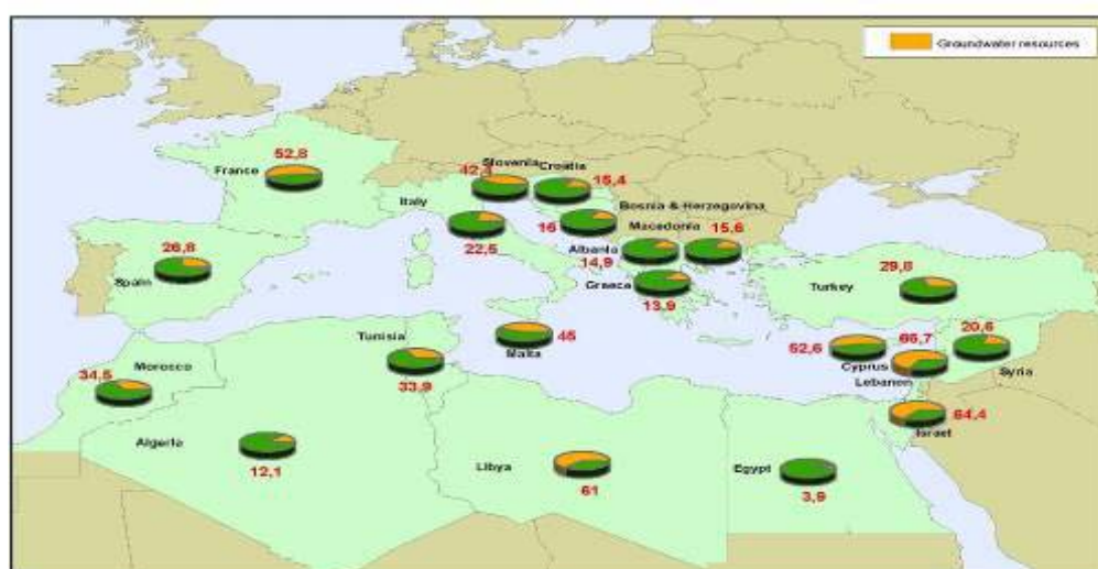
Figure 9: Natural renewable groundwater resources in Mediterranean countries % Total renewable water resources (Margat and Vallée, 2000 in Blue Plan)
