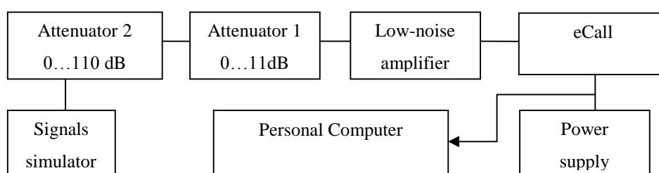
Figure 5 – Arrangement for evaluation of GNSS module sensitivity
