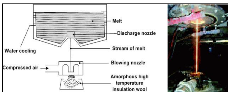
Figure 2.14 Parallel blowing method
