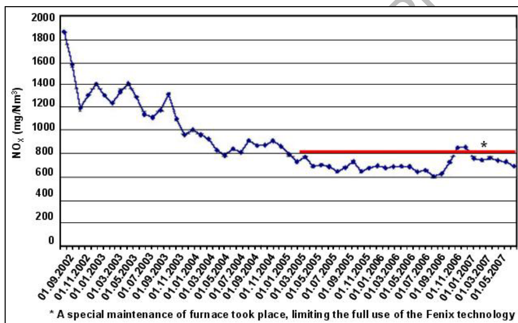
Figure 4.6: NO x emissions from the FENIX process Source: [65, GEPVP-Proposals for GLS revision 2007]
