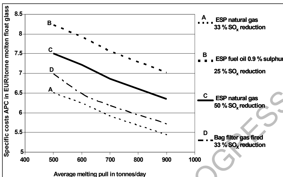
Figure 4.3: Specific costs per tonne molten glass for air pollution control by dry scrubbing and filters, with total disposal of filter dust, for float glass furnaces depending on melting pull
