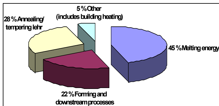
Figure 3.8: Energy usage in soda-lime-silica glass tableware production Source: [140, Domestic Glass 2008]
