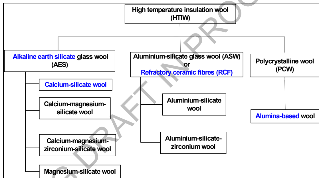
Figure 1.2: Most popular high temperature insulation wools for above 600 °C and up to 1800 °C
