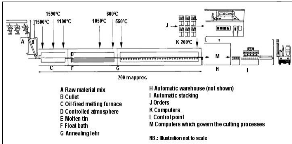
Figure 2.6: The float glass process
