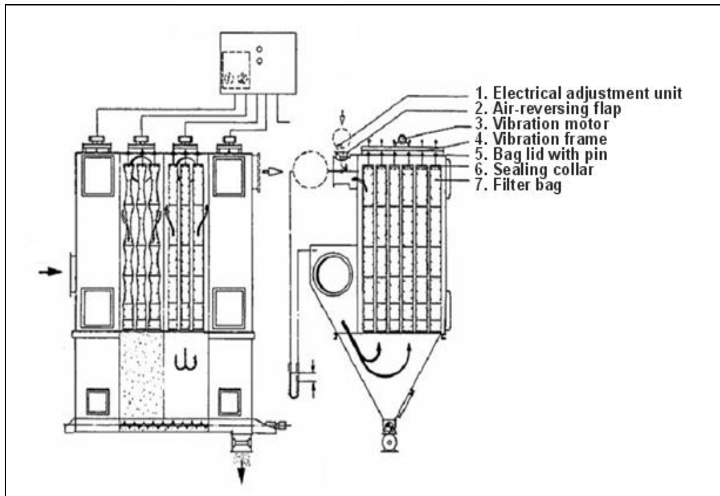
Figure 4.4: Bag (fabric) filter scheme Source: [70, VDI 3469-1 2007]
