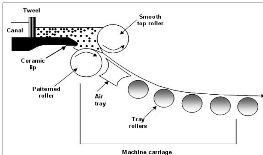
Figure 2.7: The rolled glass process
