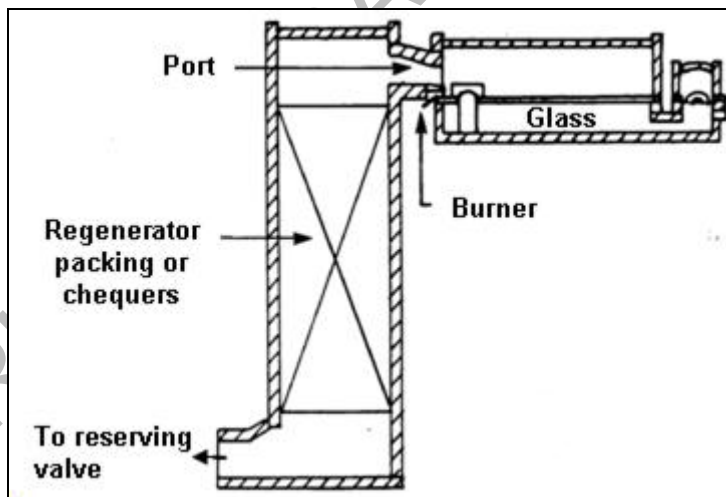
Figure 2.3: Single pass end-fired regenerative furnace
