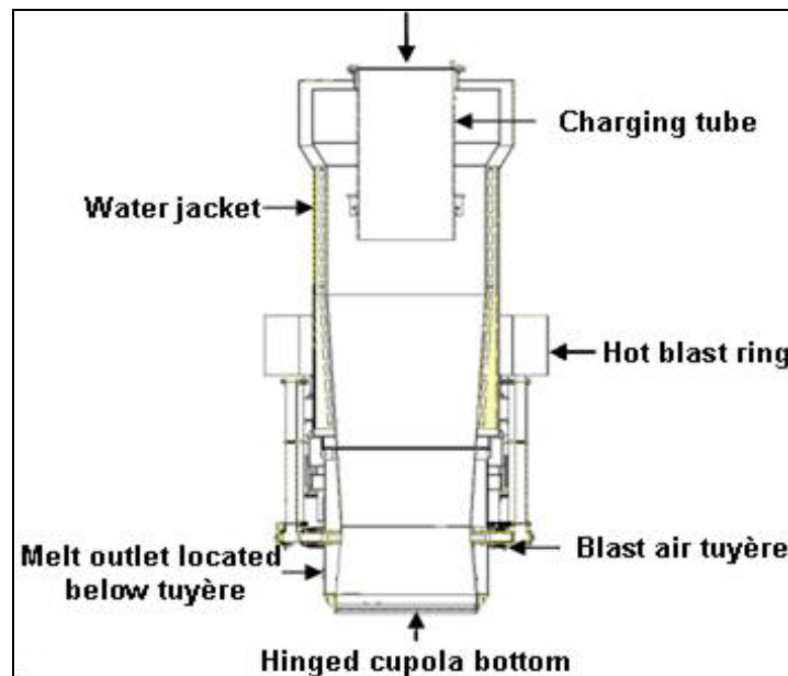
Figure 2.13 A typical hot blast cupola furnace
