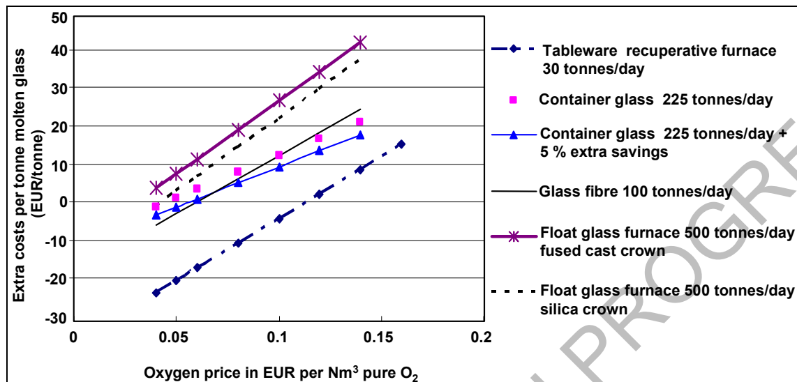
Figure 4.7: Difference in specific melting costs after conversion from conventional furnaces to oxygen-firing for different glass production installations (container, float, continuous filament glass fibre and tableware) Source: [94, Beerkens - APC Evaluation 2008]
