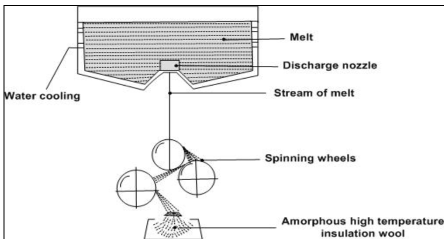
Figure 2.16: Spinning process Source: [71, VDI 3469-5 2007]
