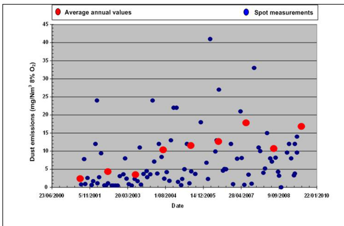
Figure 4.2 Results of dust emissions (monthly spot measurements) from an oil-fired float glass furnace equipped with an ESP and dry scrubbing with \text{Ca}(\text{OH})_2 Source: [163, Glass for Europe 2009]
