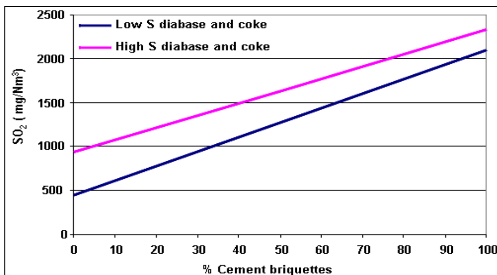
Figure 3.9: Expected concentration of SO 2 depending on the percentage of cement briquettes recycled with the batch charge in the cupola furnace Source: [89, EURIMA Suggestions 2007]
