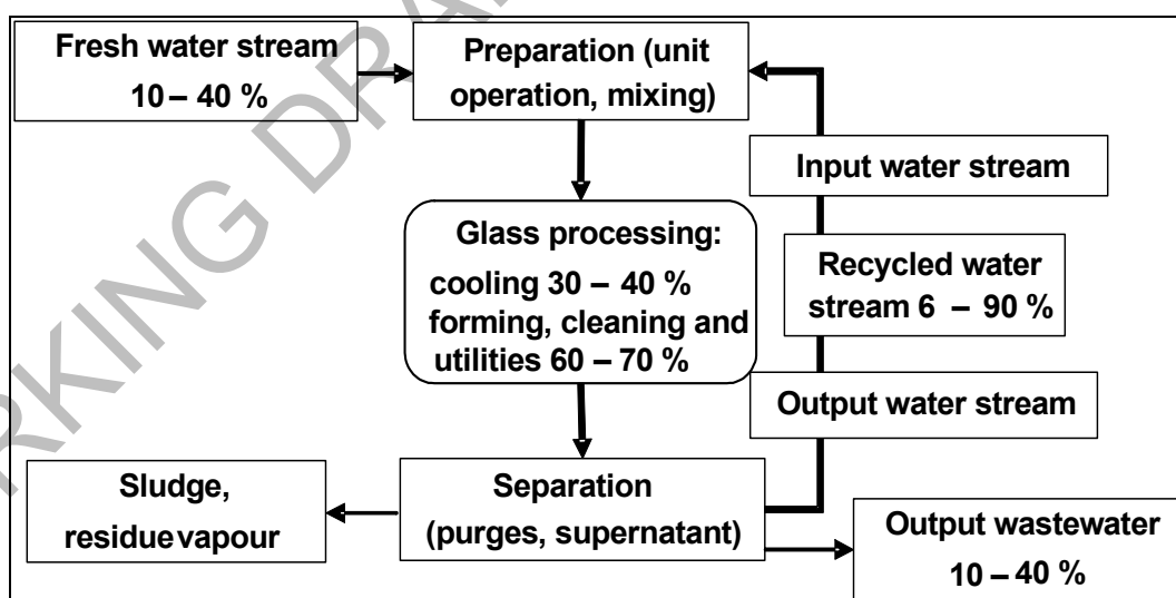
Figure 3.1: Typical water distribution in a container glass plant
