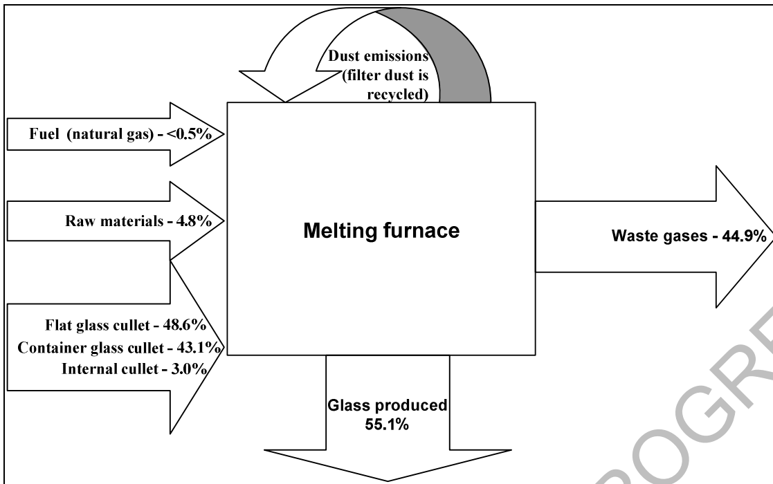
Figure 8.3: Schematic sulphur balance for an oxy-fuel glass wool furnace with filter dust recycling Source: [136, EURIMA 2008]
