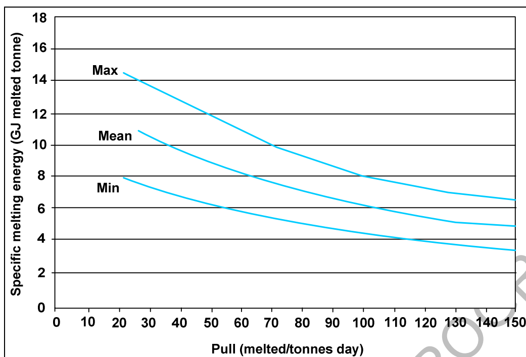
Figure 3.2: Trend curves for the total melting energy in flaconnage production from the FEVE survey (2005 data—primary energy for electric boosting or oxygen production is not included) Source: [126, FEVE 2009]v
