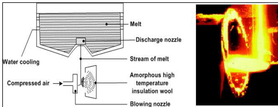
Figure 2.15: Horizontal blowing method Source: [71, VDI 3469-5 2007]
