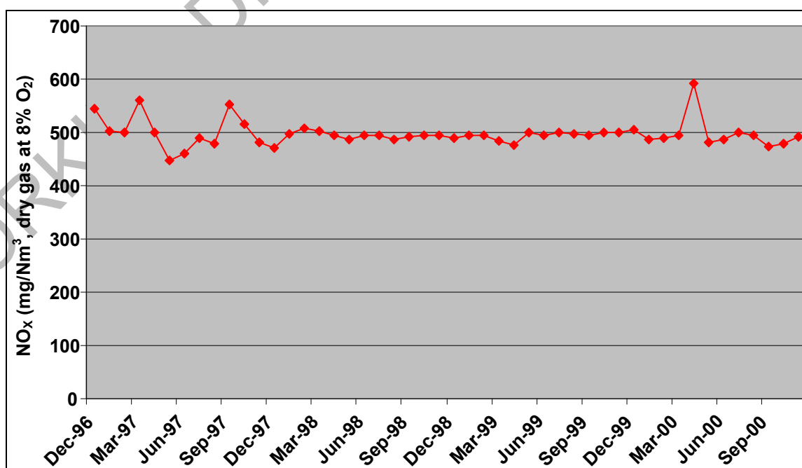
Figure 4.8: Variation of NO x concentration over time for a float glass furnace equipped with SCR
