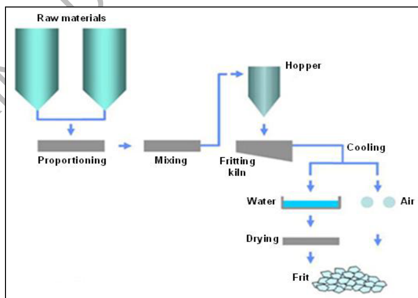
Figure 2.17: Schematic representation of the frits production process
