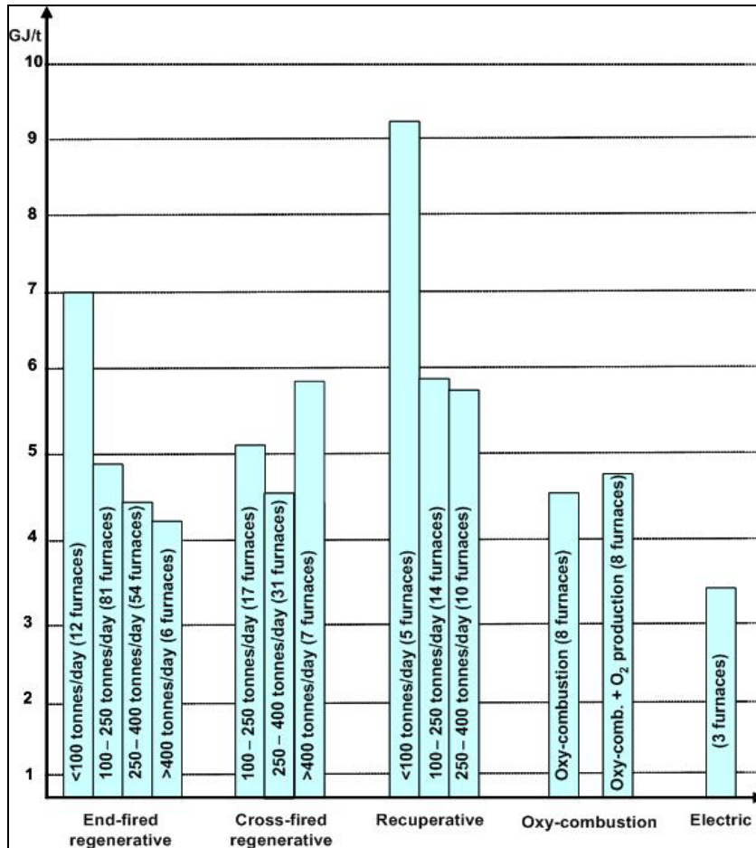
Figure 3.4: Mean energy consumptions in glass container furnaces expressed in GJ/tonne melted glass and standardised to 50 % cullet (2005) Source: [64, FEVE 2007]
