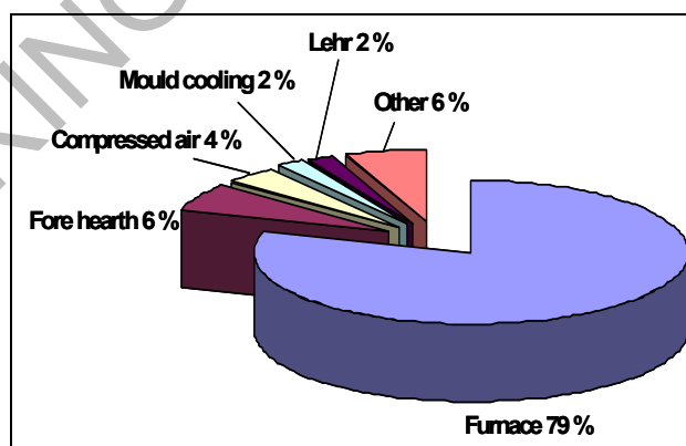
Figure 3.3: Energy usage in a typical bottle/jar container glass plant ( not representative of perfume/cosmetic ware production )
