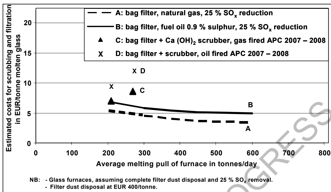
Figure 4.5: Estimated costs for dry scrubbers in combination with bag filters for container glass furnaces, assuming a complete filter dust disposal and 25 % SO x removal Source: [94, Beerkens - APC Evaluation 2008]
