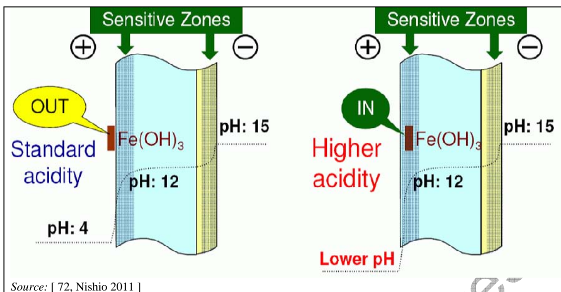
Figure 4.9: Effect of pH value on the location of iron hydroxide precipitation in membranes
