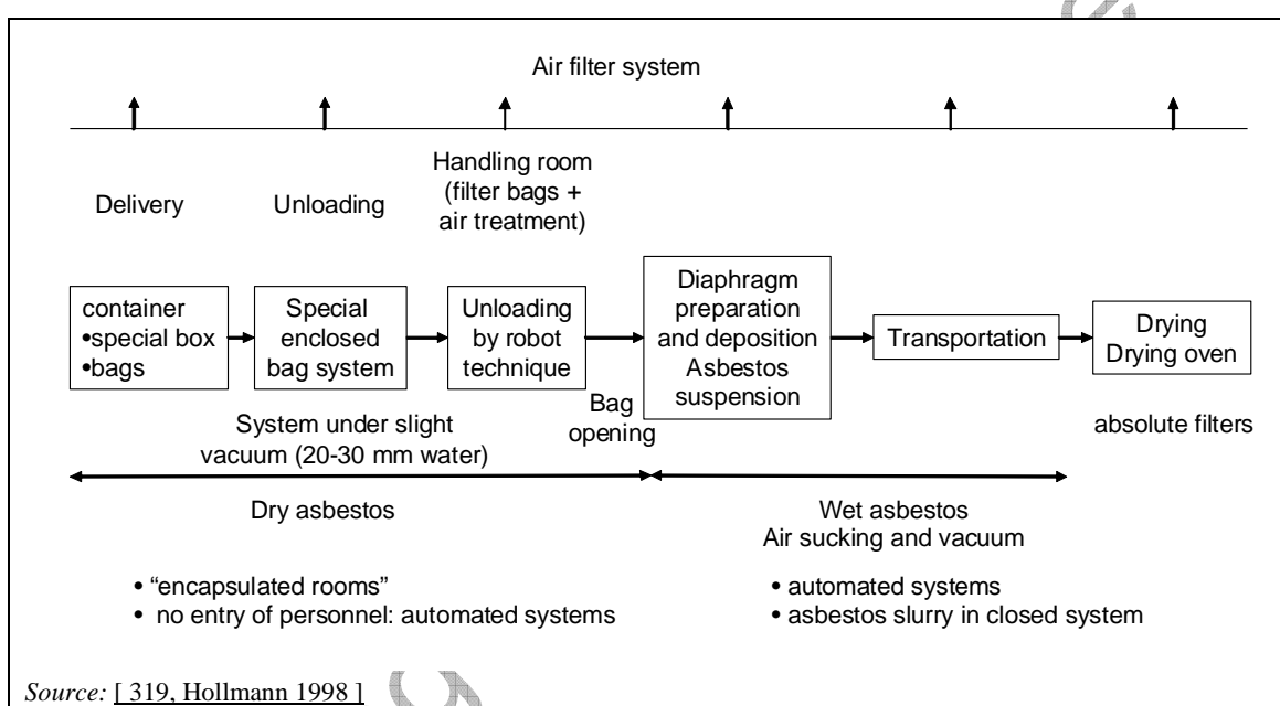
Figure A.0.1: Example of handling of asbestos at the Dow plant in Stade (Germany)
