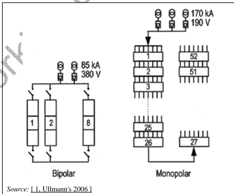
Figure 2.14: Electrolyser architecture
