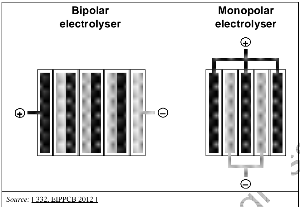
Figure 2.13: Simplified scheme of monopolar and bipolar electrolyzers
