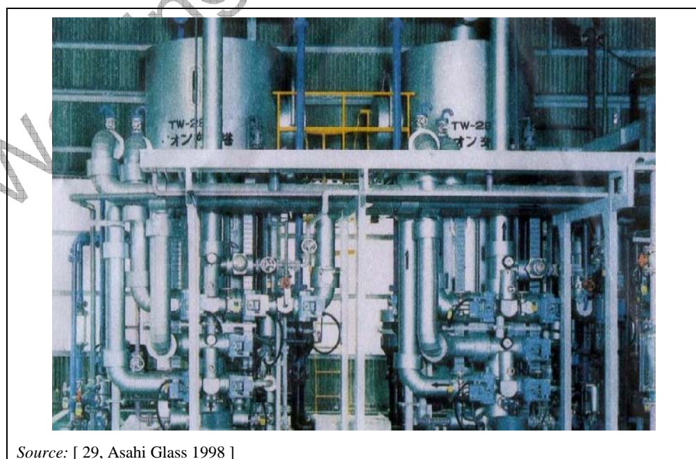
Figure 2.17: View of chelate resin towers in a secondary brine purification system
