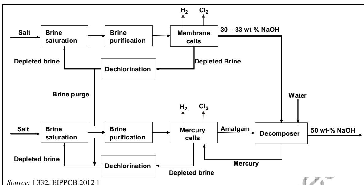
Figure 2.8: Flow diagram of the integration of the membrane and mercury cell techniques
