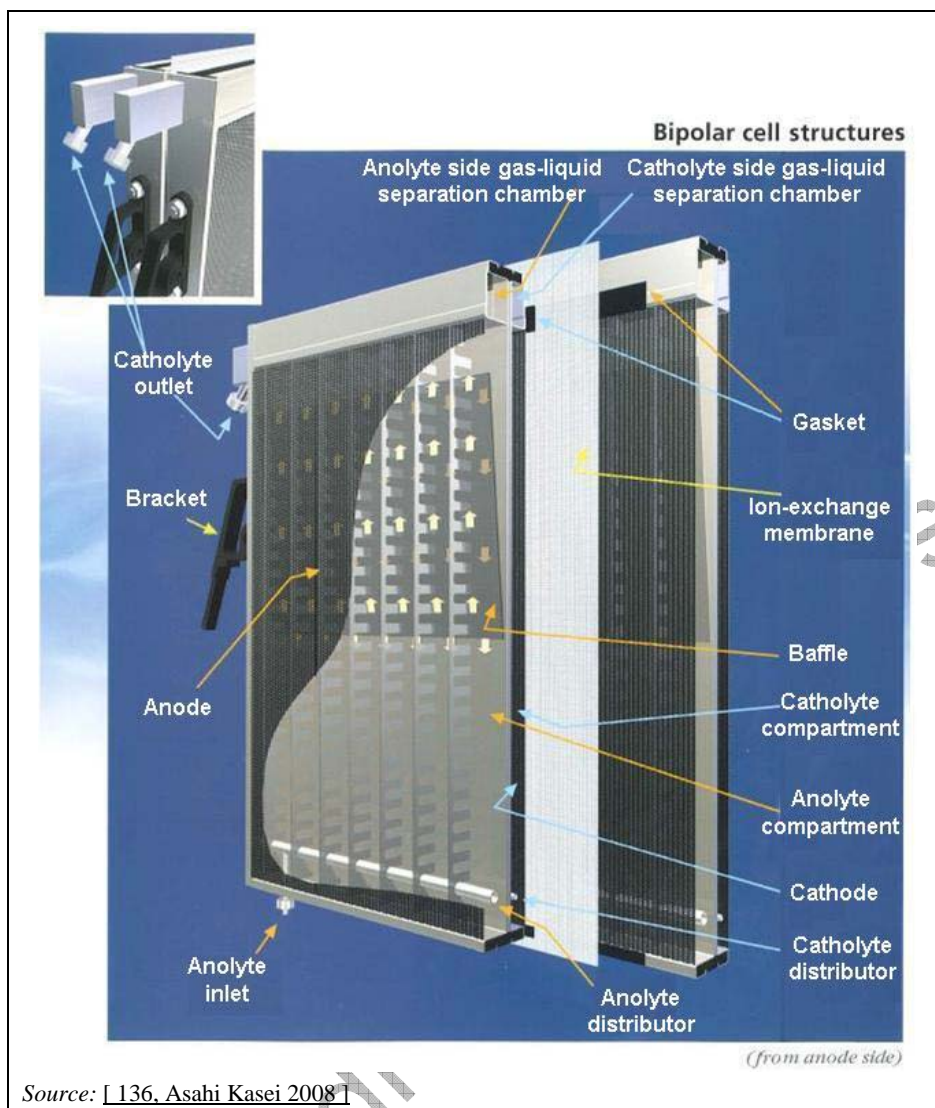
Figure 2.9: Schematic view of a typical bipolar membrane electrolysis cell
