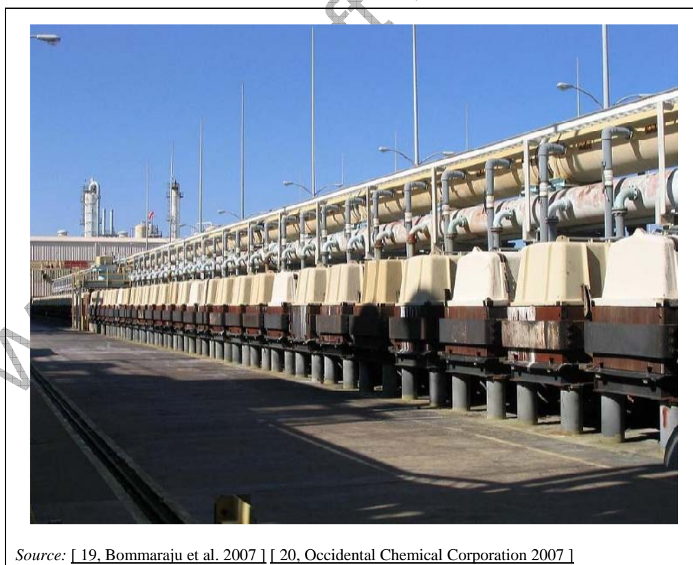
Figure 2.7: View of an open-air diaphragm cell room equipped with monopolar electrolyzers
