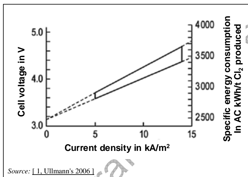
Figure 3.1: Cell voltage and specific electrical energy consumption versus cell current density for the mercury cell technique
