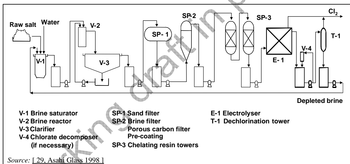
Figure 2.15: Flow diagram of a possible layout for the brine system used in the membrane cell technique
