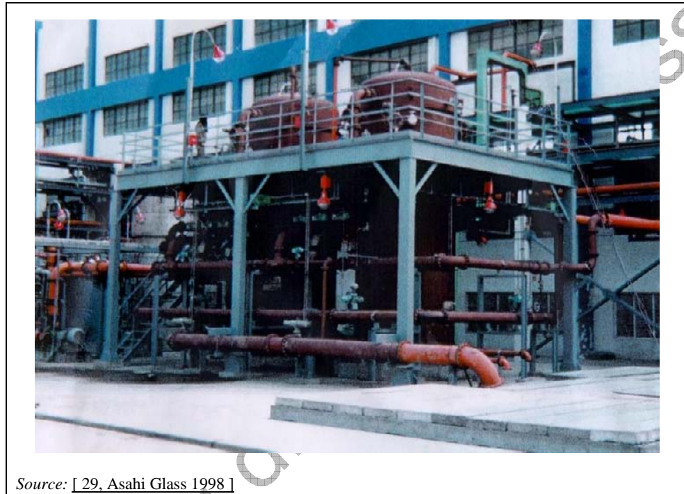
Figure 2.16: View of polishing filters in a secondary brine purification system
