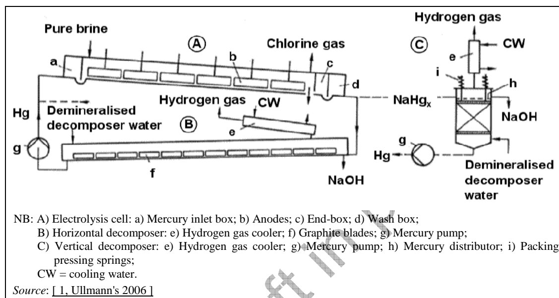
Figure 2.3: Schematic view of a mercury electrolysis cell with horizontal and vertical decomposer
