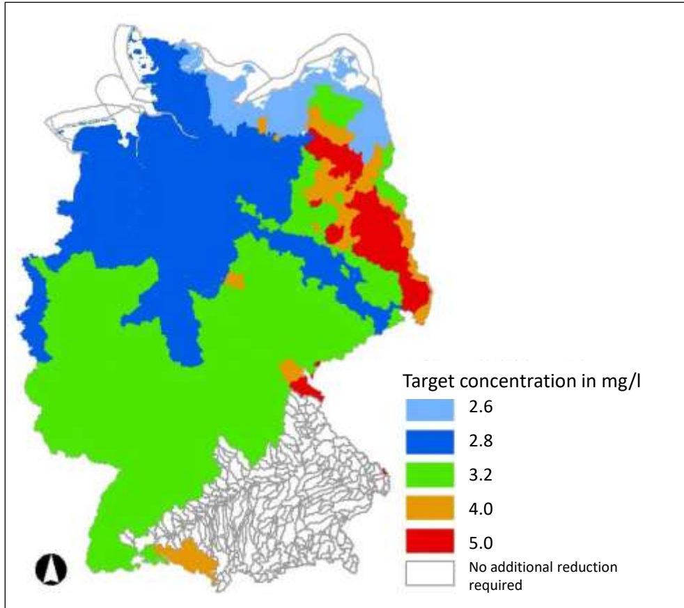
Figure 5-4: Mean annual target concentration for total nitrogen (in mg L -1 ) that is required in the catchments of German rivers in order to achieve good status with respect to eutrophication in coastal and marine waters of the North Sea and Baltic Sea. At the time that this work was performed no nutrient reduction targets had been set for the Black Sea, into which the Danube catchment drains (LAWA 2016) (but see 5.5.2 for recent developments).
