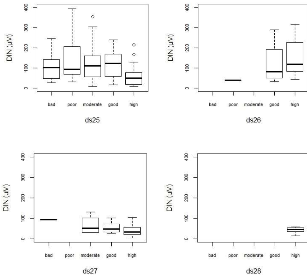
Figure 7-3: DIN concentrations (µM) between status classes for each data set (ds) separately: ds25 (Ireland, Netherlands, United Kingdom), ds26 (FR), ds27 (ES) and ds28 (PT).
