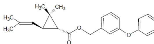
1-R-trans-Phenothrin
