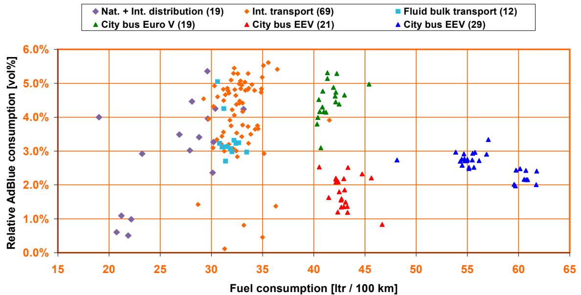
Figure 20: Fuel and AdBlue consumption per fleet (166 vehicles)
