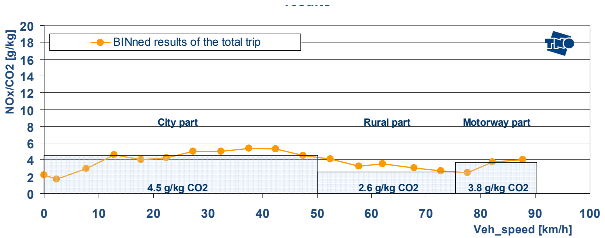
Figure 4: Emissions in the different parts of the Euro VI trip compared with the binned results - Vehicle I
