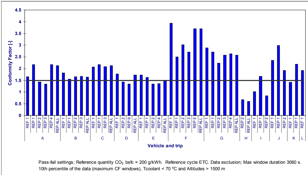
Figure 18: The NOx conformity factors of the vehicles tested. Results are shown for a reference trip (REF 1), for representative sub-trips (REP 1, 2, 3...) and for complete representative trips (REP ALL).
