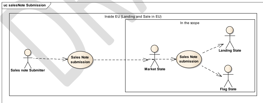
Use Case Submission diagram
