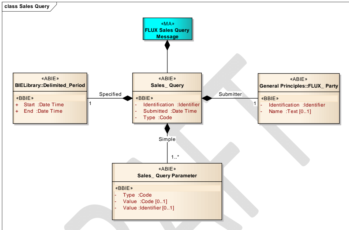
Class Diagram for Sales Query message.
