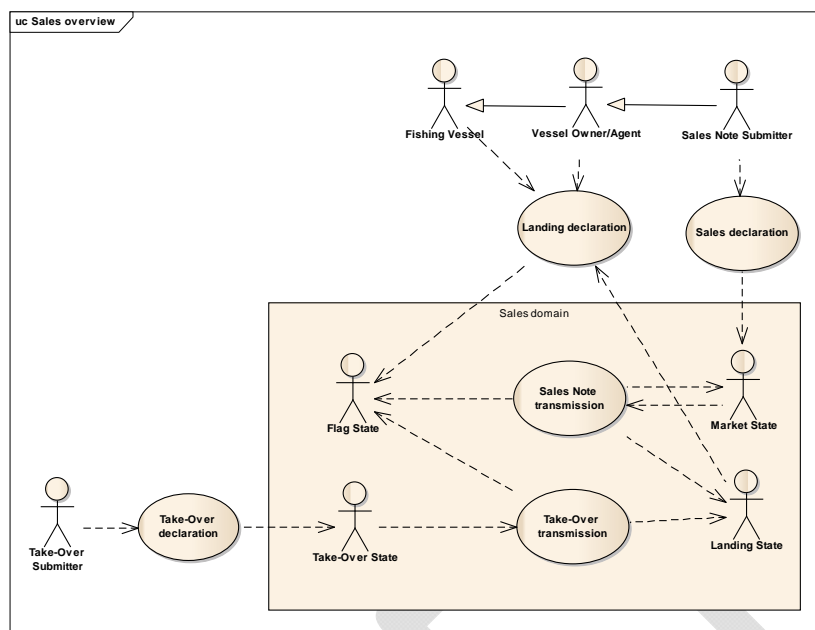
Sales domain: Sales overview diagram.
