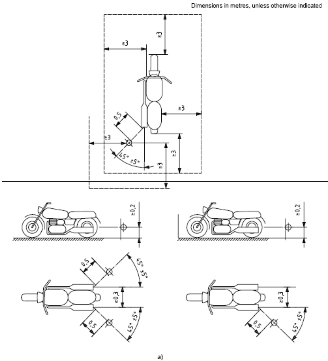
Figure 2 Measuring positions for stationary mopeds
