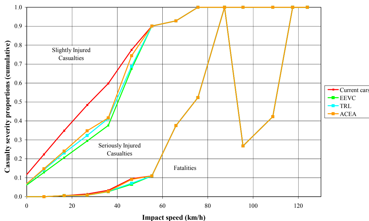
Figure 4.1. Injury severity risk by impact speed using banded data
