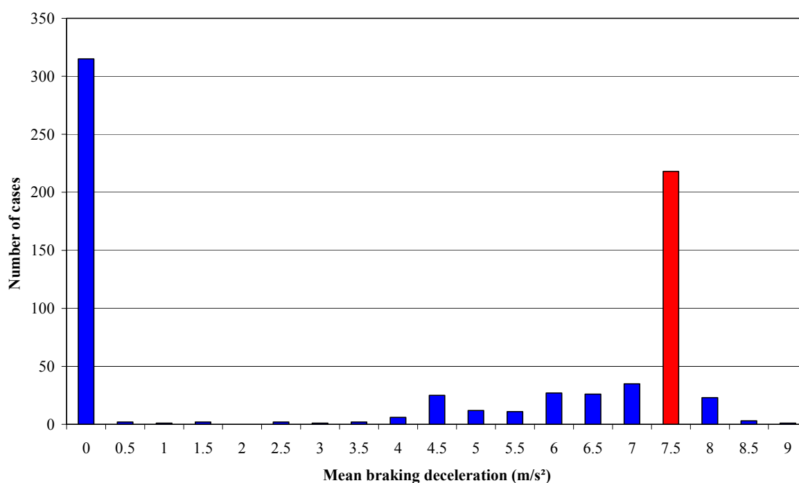
Figure 3.1. Number of cases in BAS database by mean braking deceleration
