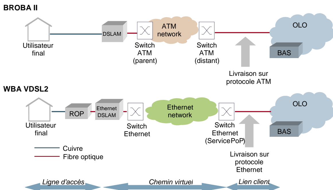
Figure 6.1 : Offres Belgacom BROBA II & WBA VDSL2 [Source: Analysys Mason, Belgacom]
